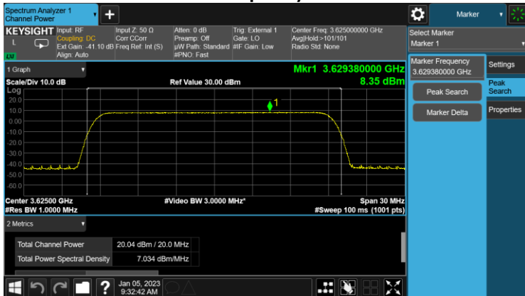
20MHz BW, TM1.1 Channel Frequency 3625MHz
