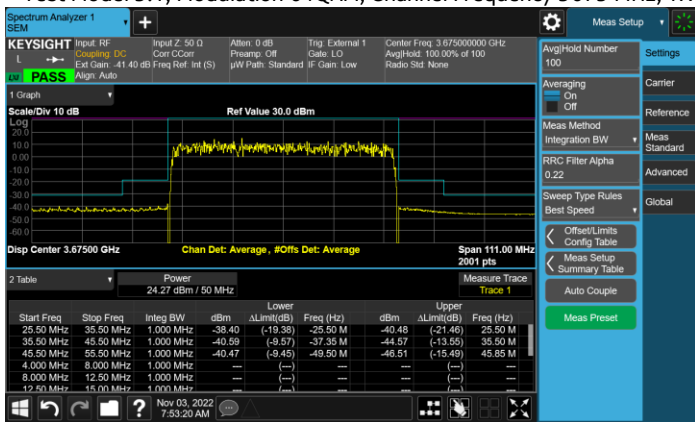
Test Model 3.1, Modulation 64QAM, Channel Frequency 3675 MHz, TX1
