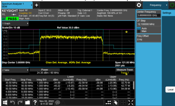
Test Model 3.1a, Modulation 256QAM, Channel Frequency 3670 MHz, TX1
