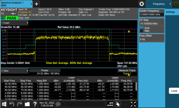
Test Model 3.1, Modulation 64QAM, Channel Frequency 3590 MHz, TX0
