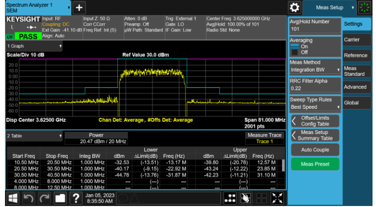
Test Model 3.2, Modulation QPSK/16QAM, Channel Frequency 3625MHz, TX3
