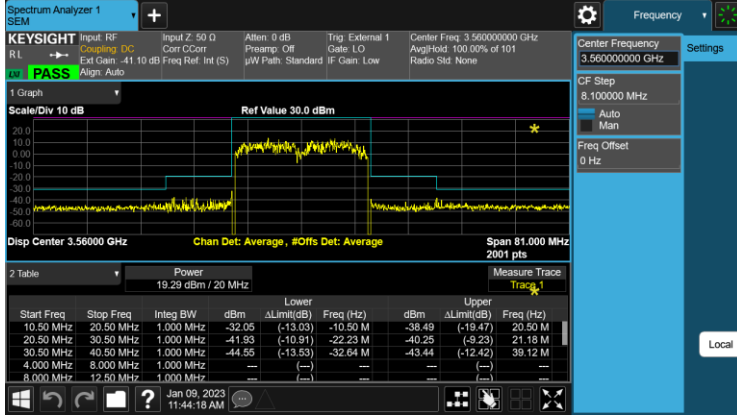
Test Model 3.2, Modulation QPSK/16QAM, Channel Frequency 3555+3565MHz, TX3
