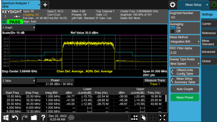
Test Model 3.1a, Modulation 256QAM, Channel Frequency 3685 MHz, TX1
