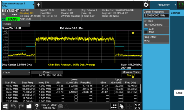
Test Model 3.1a, Modulation 256QAM, Channel Frequency 3655 MHz, TX1
