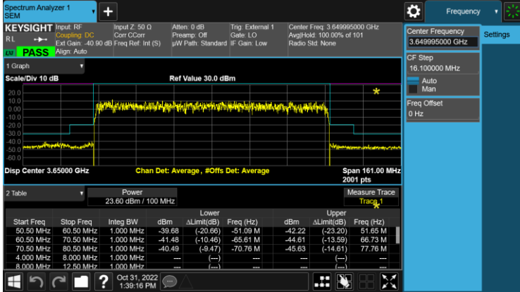
Test Model 3.1a, Modulation 256QAM, Channel Frequency 3650 MHz, TX0
