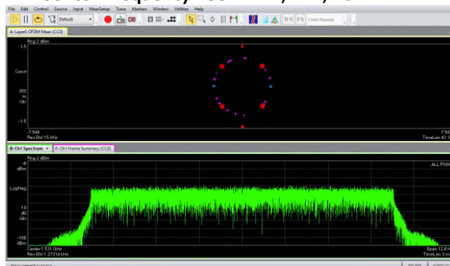
Modulation QPSK TM1.1 Center Frequency 1531 MHz, LTE, 10MHz BW
