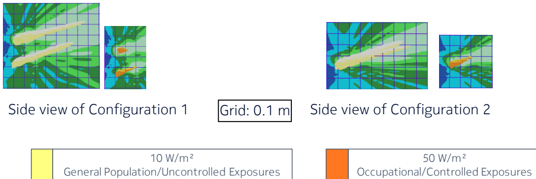
Figure 10 – Power density from AWEWA/B (or FA3WA) for the actual maximum transmitted power of 0.4 W (corresponding to the actual EIRP threshold of 49.52 dBm) and the beam oriented in azimuth = 0° & elevation = -20°, together with the power density from FA3UB (or AWEUC/D) for the actual maximum transmitted power of 0.2 W (corresponding to the actual EIRP threshold of 49.52 dBm) and the beam oriented in azimuth = 0° & elevation = -15°
