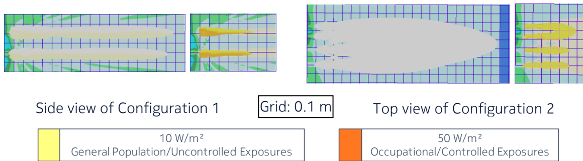
Figure 3 – Power density from AWEWA/B (or FA3WA) for the time-averaged maximum transmitted power of 1.42 W (corresponding to the time-averaged maximum EIRP of 55.52 dBm) and the beam oriented in azimuth = 0° & elevation = 0°, together with the power density from FA3UB (or AWEUC/D) for the time-averaged maximum transmitted power of 0.76 W (corresponding to the time-averaged maximum EIRP of 55.52 dBm) and the beam oriented in azimuth = 0° & elevation = 0°
