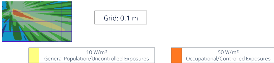
Figure 6 – Side view of the power density for the time-averaged actual maximum transmitted power of 0.36 W and the beam oriented in azimuth = 0° & elevation = +20°
