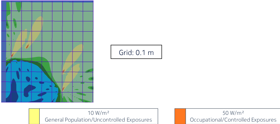
Figure 10 – Top view of the power density for the time-averaged actual maximum transmitted power of 0.36 W and the beam oriented in azimuth = -60°/+60° & elevation = 0°
