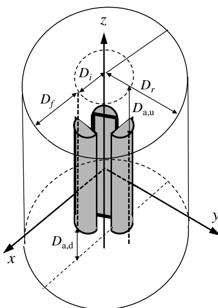
Figure 1 – Shape of the compliance boundary used for the RF exposure compliance assessment (from [4]).
