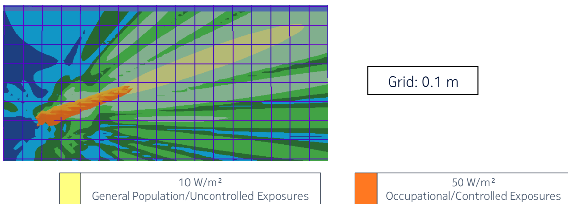
Figure 7 – Side view of the power density for the time-averaged maximum transmitted power of 1.42 W and the beam oriented in azimuth = 0° & elevation = -20°
