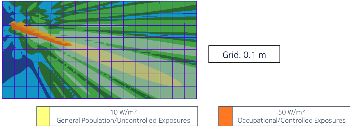
Figure 5 – Side view of the power density for the time-averaged maximum transmitted power of 1.42 W and the beam oriented in azimuth = 0° & elevation = +20°
