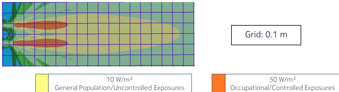
Figure 3 – Top view of the power density for the time-averaged maximum transmitted power of 1.42 W and the beam oriented in azimuth = 0° & elevation = 0°
