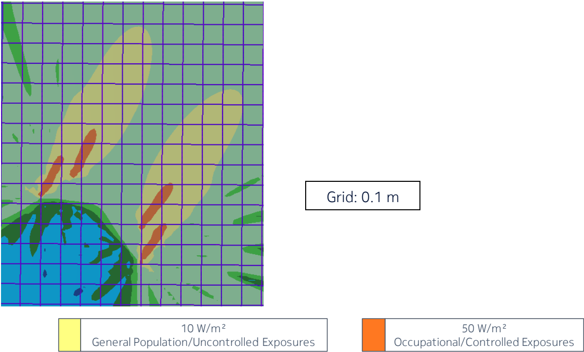
Figure 9 – Top view of the power density for the time-averaged maximum transmitted power of 1.42 W and the beam oriented in azimuth = -60°/+60° & elevation = 0°
