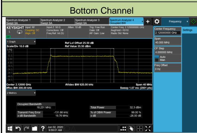
20MHz Channel Bandwidth - Carrier Position -9097.5 kHz
