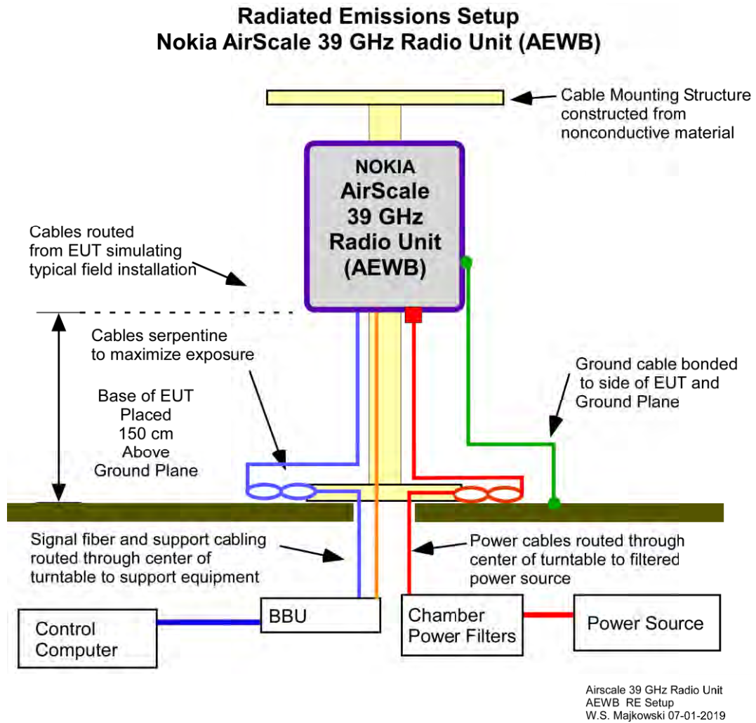
Figure 3.5 Radiated Emissions Product Setup
