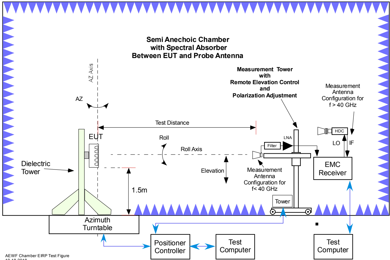
Figure 3.1.1 Test Set-Up for Measurement of Radio Transmitter Performance
