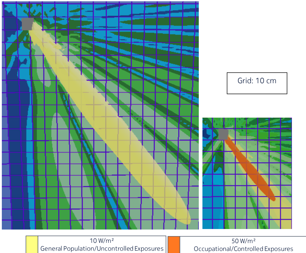
Figure 8 – Side view of AEUB power density for the time-averaged maximum transmitted power of 1.33 W and the beam oriented in azimuth = 0° & elevation = -45°
