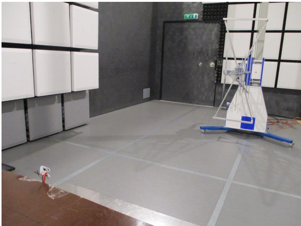
Figure 2: Spurious emission 200 MHz-1000 MHz
