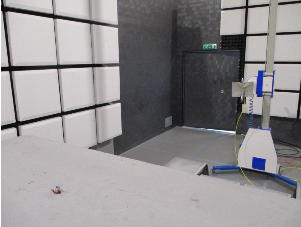
Figure 3: Spurious emission 1-18 GHz
