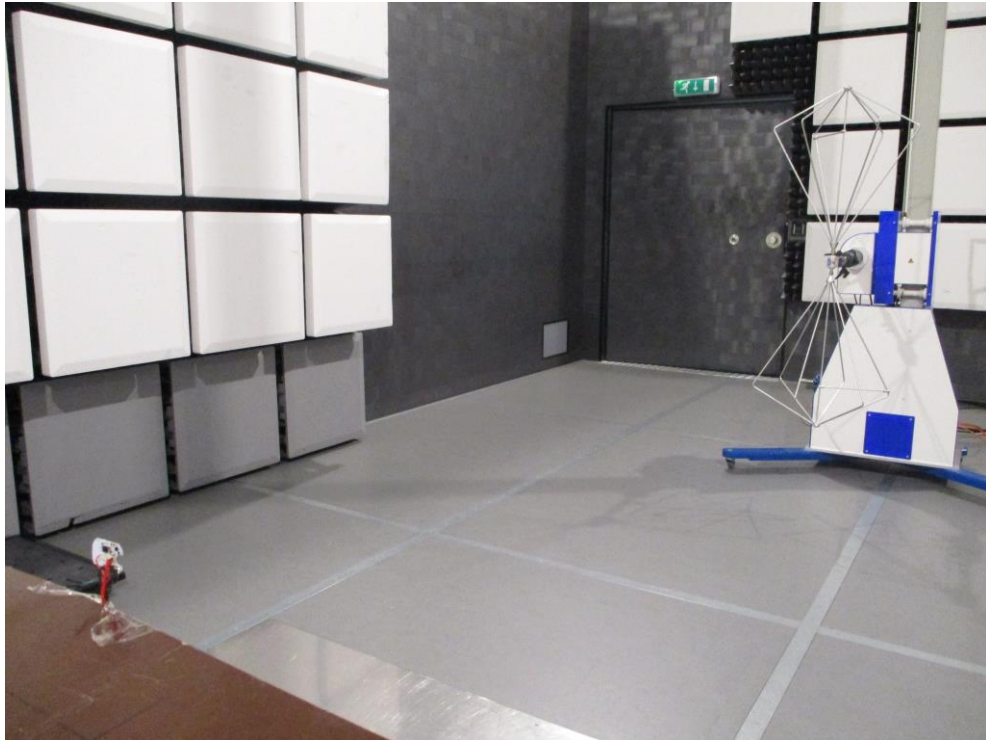
Figure 1: Spurious emission 30 MHz-200 MHz
