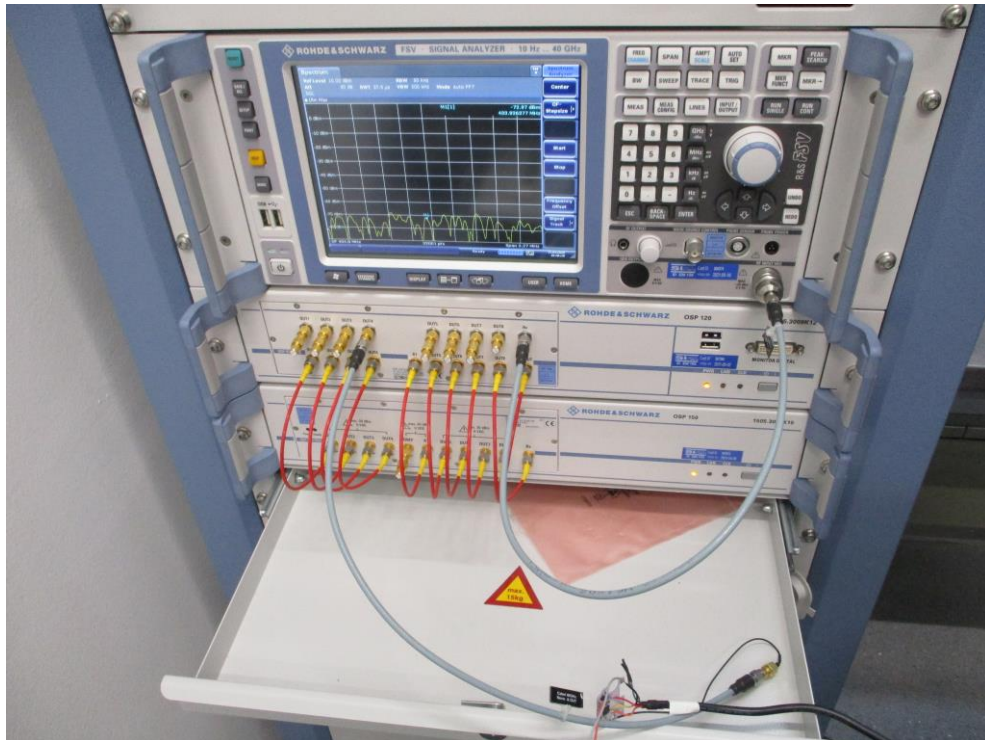
Figure 11: Conducted measurements test setup
