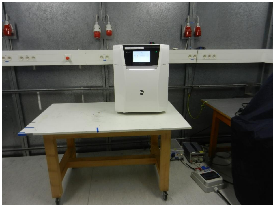
Figure 8 – Test setup for AC Power Line Conducted Emissions
