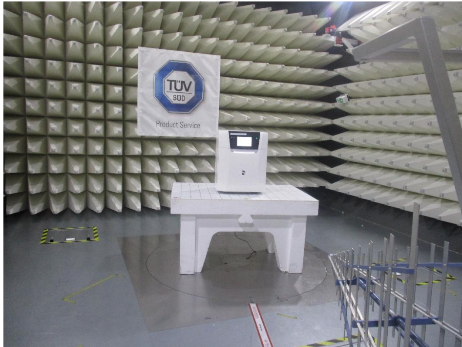
Figure 3 – Test setup for radiated emission
