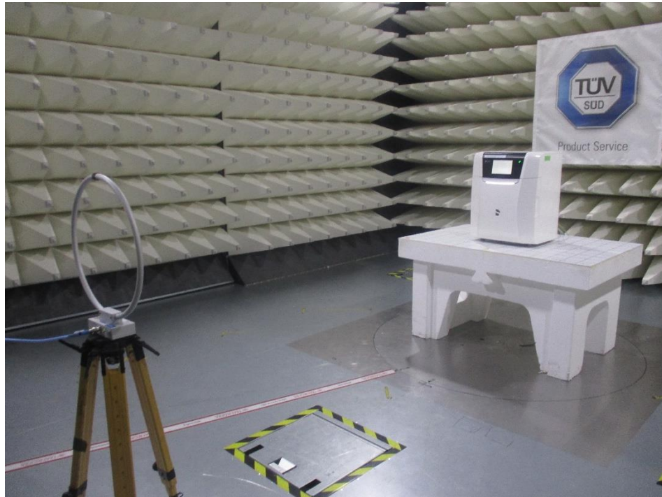
Figure 5 – Test setup for radiated emission 9kHz – 30MHz
