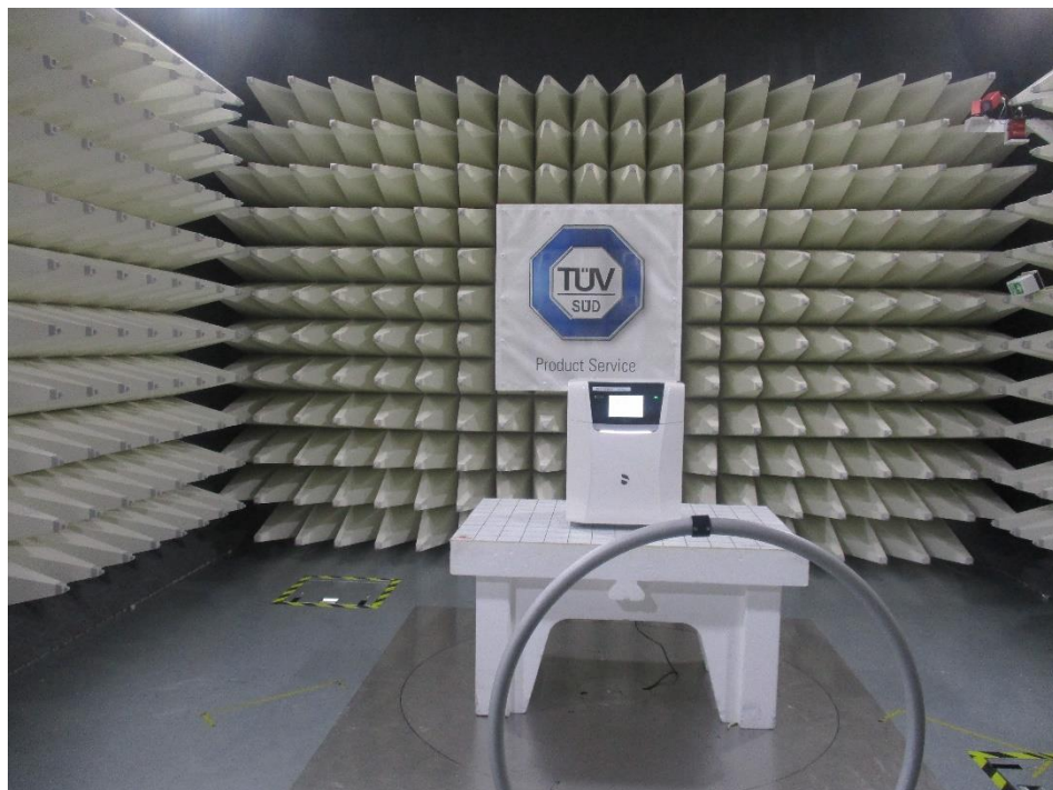
Figure 6 – Test setup for radiated emission 9kHz – 30MHz
