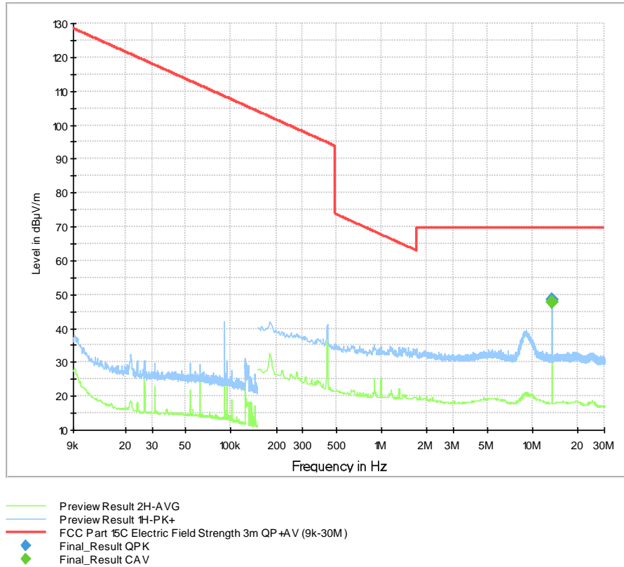
Figure 4 – 9kHz to 30MHz
