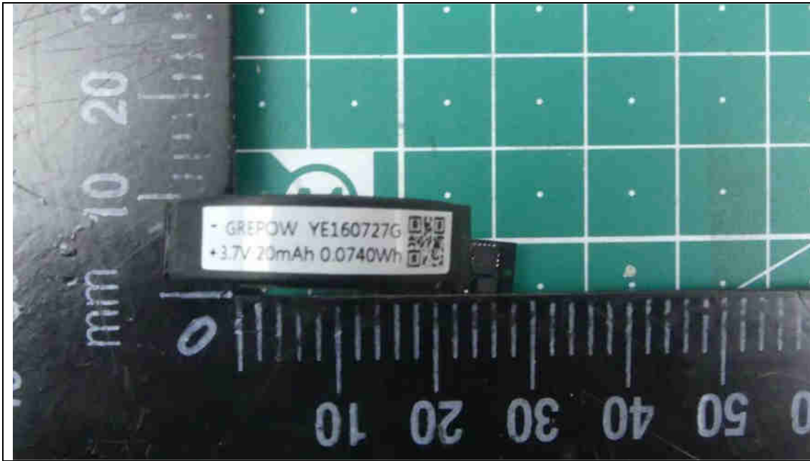
BATTERY DETAILS
