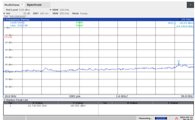
Conducted Emissions BLE 2402 MHz, 2Mb, 10000-26000 MHz
