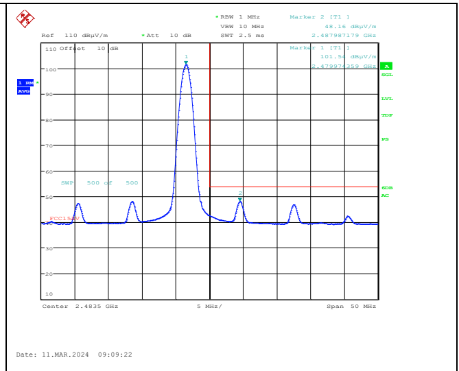
Upper Band Edge, 2480 MHz, 1Mb, Average
