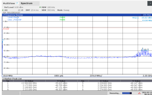
Conducted Emissions BLE 2402 MHz, 2Mb, 10-2350 MHz
