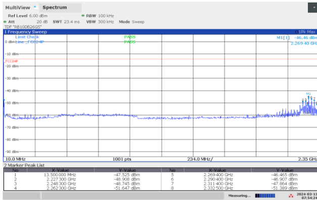
Conducted Emissions Snobee 2440 MHz, 10-2350 MHz
