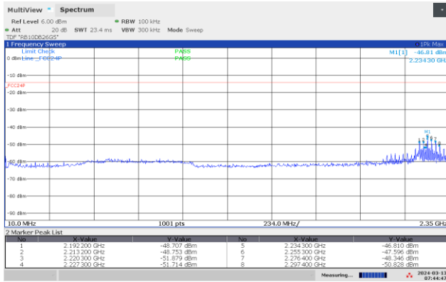
Conducted Emissions Snobee 2405 MHz, 10-2350 MHz
