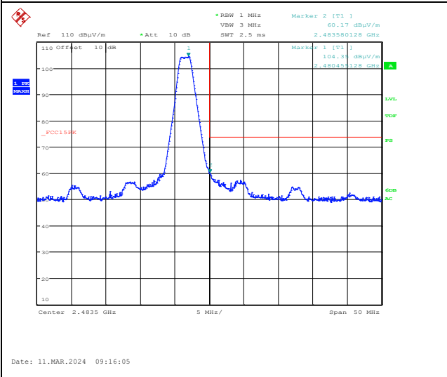
Upper Band Edge, 2480 MHz, BLE 2Mb, Peak
