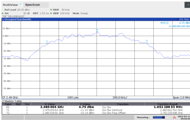
High channel 99% Occupied BW, BLE 1Mb
