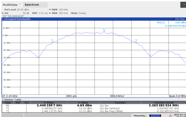
Mid channel 99% Occupied BW, Snobee
