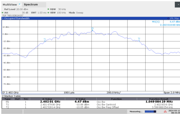
Low channel 99% Occupied BW, BLE 1Mb
