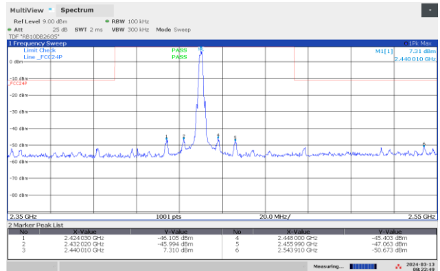
Conducted Emissions BLE 2440 MHz, 2Mb, 2350-2550 MHz
