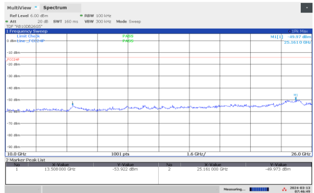
Conducted Emissions Snobee 2405 MHz, 10000-26000 MHz
