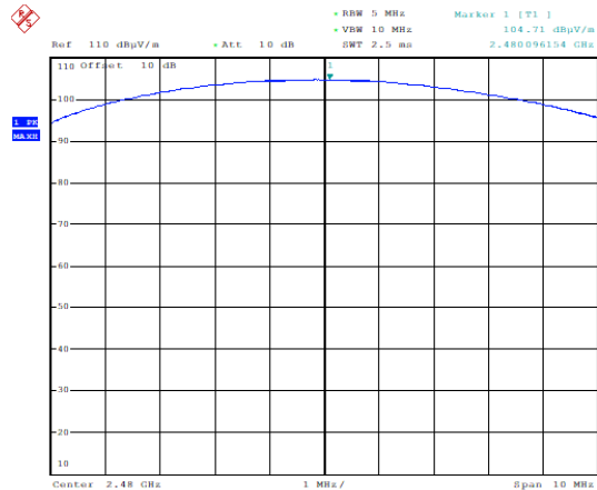
BLE 1Mb, Peak Field Strength, 2480 MHz
