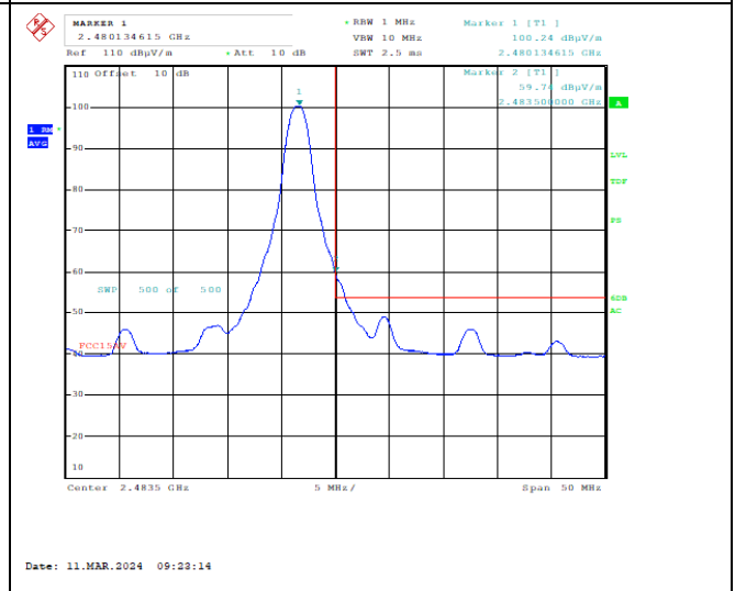
Upper Band Edge, 2480 MHz, Snobee, Average
