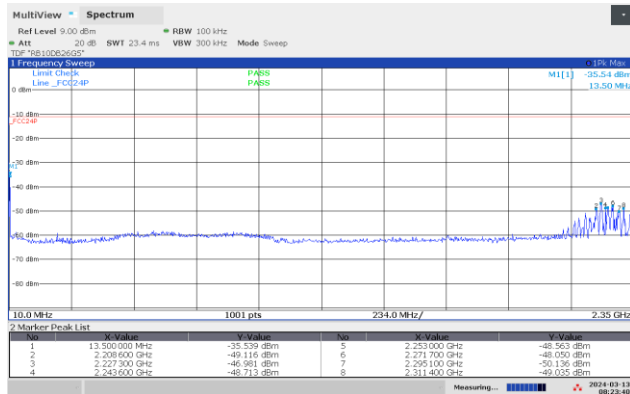
Conducted Emissions BLE 2440 MHz, 2Mb, 10-2350 MHz
