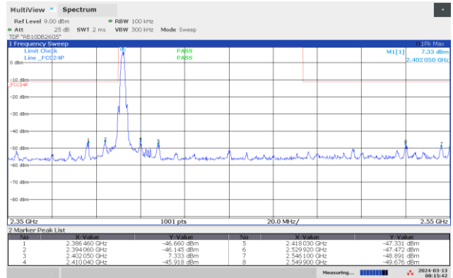
Conducted Emissions BLE 2402 MHz, 2Mb, 2350-2550 MHz
