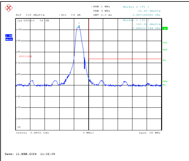
Upper Band Edge, 2480 MHz, BLE 1Mb, Peak
