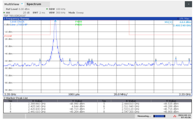
Conducted Emissions Snobee 2405 MHz, 2350-2550 MHz
