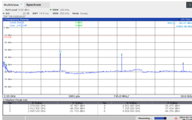
Conducted Emissions BLE 2402 MHz, 2Mb, 2550-10000 MHz
