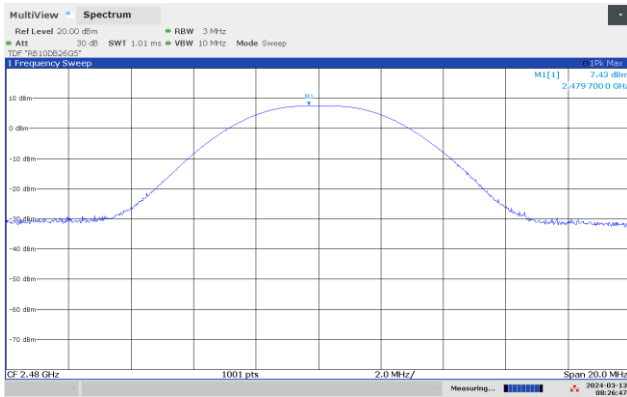
BLE 1Mb, Peak Power, 2480 MHz
