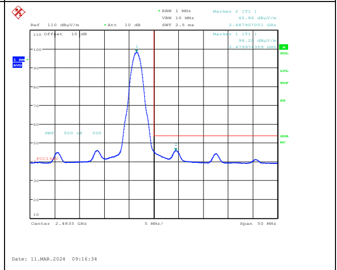
Upper Band Edge, 2480 MHz, BLE 2Mb, Average
