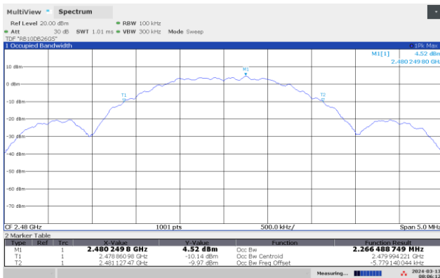
High channel 99% Occupied BW, Snobee
