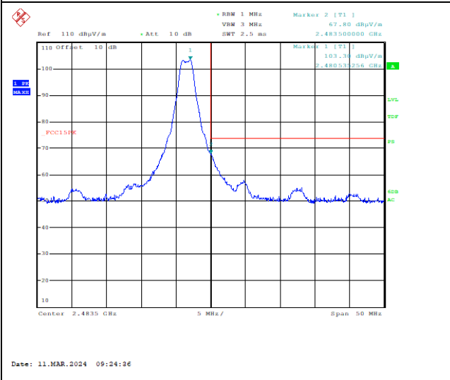
Upper Band Edge, 2480 MHz, Snobee, Peak
