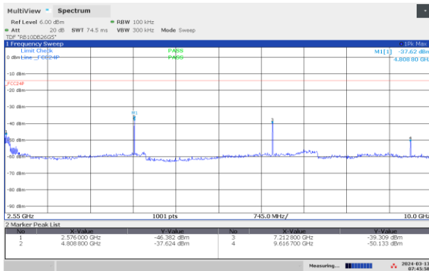
Conducted Emissions Snobee 2405 MHz, 2550-10000 MHz
