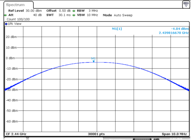
Channel 19 (2440MHz)
