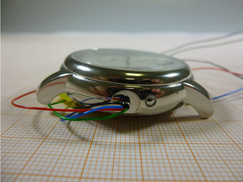
Photo 3: EUT right side view
