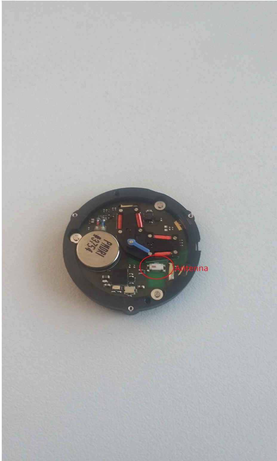
Photo 5: PCB front side view with antenna
