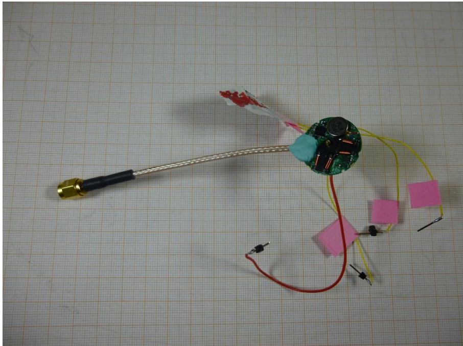
Photo 2: Conducted EUT
