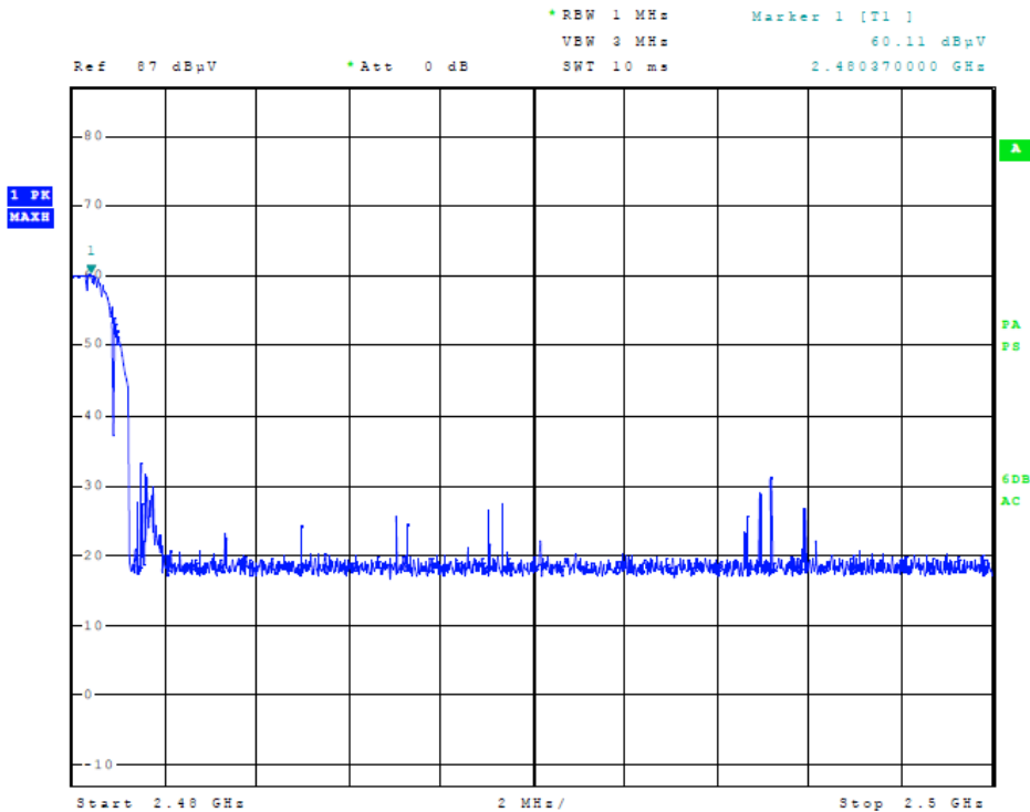
Figure 8 Plot of Transmitter Emissions (High Band Edge)
