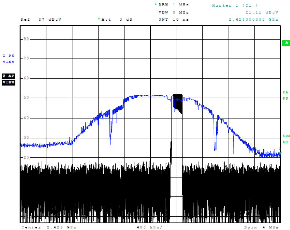
Figure 4 Plot of Transmitter Emissions (In 2402-2480 MHz band, 2426)
