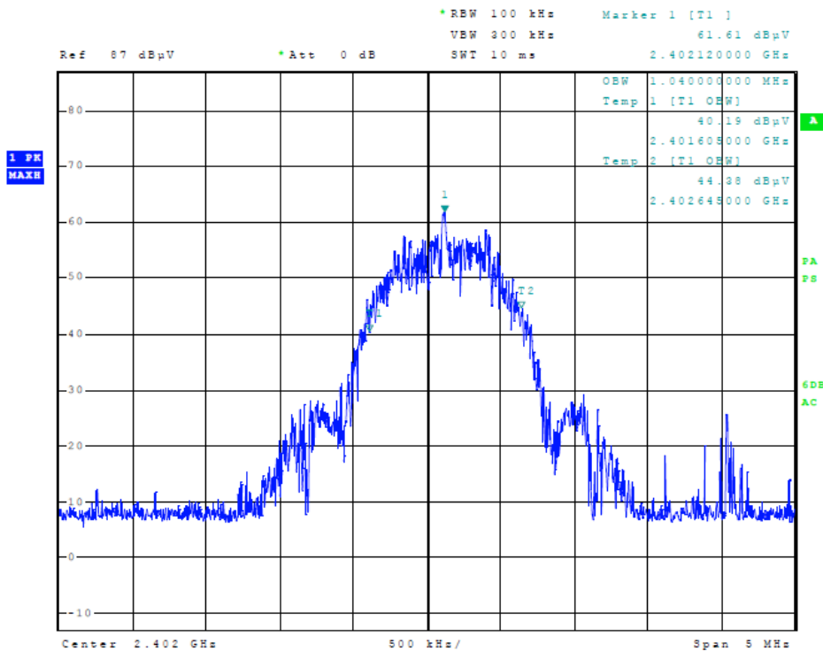
Figure 6 Plot of Transmitter Emissions (2402-2480 MHz, 99% Occupied Bandwidth)
