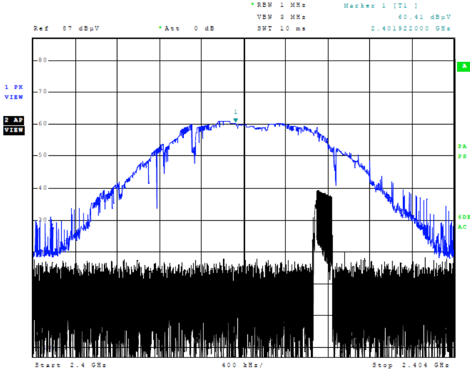
Figure 3 Plot of Transmitter Emissions (In 2402-2480 MHz band, 2402)
