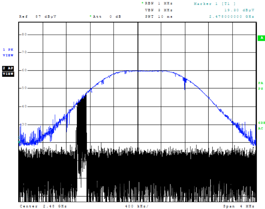
Figure 5 Plot of Transmitter Emissions (In 2402-2480 MHz band, 2480)
