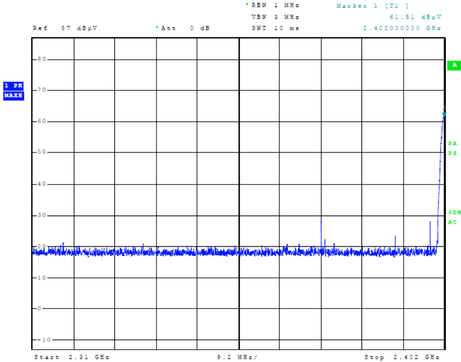
Figure 7 Plot of Transmitter Emissions (Low Band Edge)
