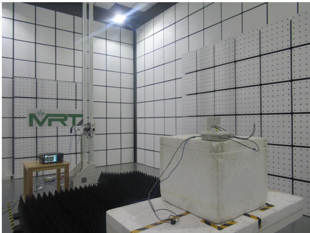
Description: Radiated Spurious Emission Test Setup for Above 18GHz (AX52)
