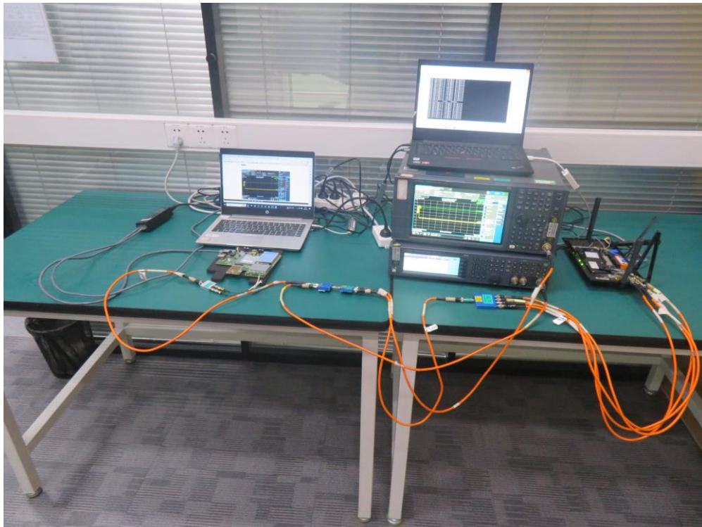
Description: Dynamic Frequency Selection Test Setup(Client Without Radar Detection)
