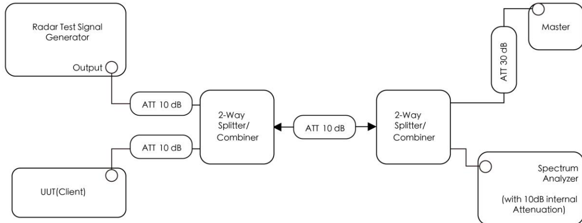
Figure 3-2: Conducted Test Setup where UUT is a Client and Radar Test Waveforms are injected into the Masters
