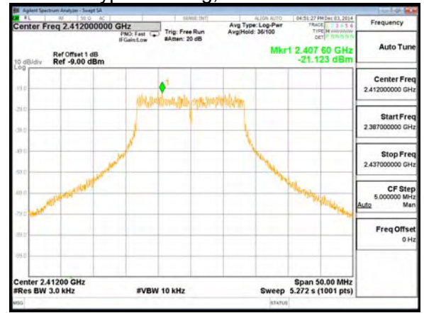
Modulation Type: 802.11g, CH01 Chain 1
