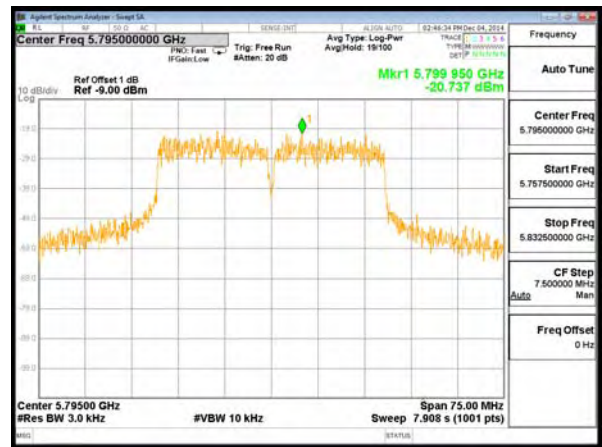
Modulation Type: 802.11n HT40,CH159 Chain 1
