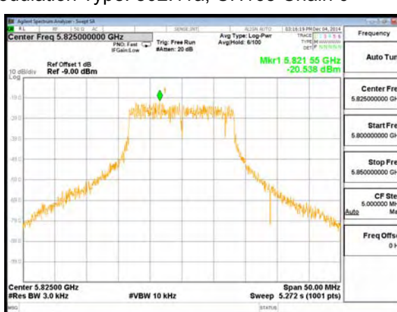
Modulation Type: 802.11a, CH165 Chain 0
