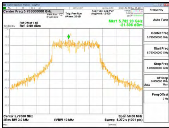
Modulation Type: 802.11n HT20 CH157 Chain 0
