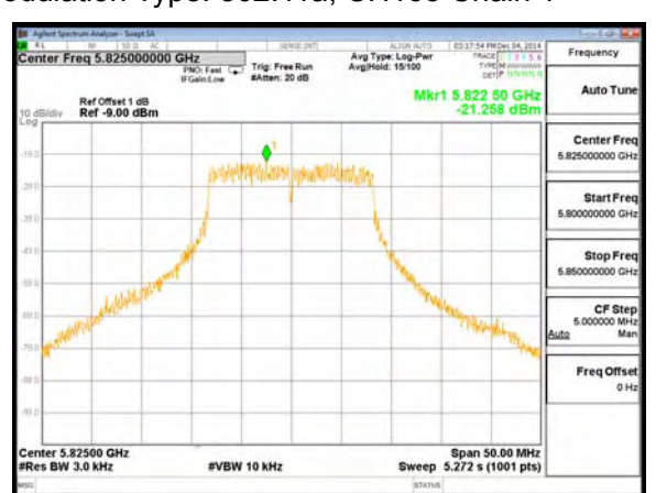
Modulation Type: 802.11a, CH165 Chain 1
