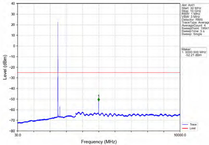
Band7_5MHz_16QAM_LCH_2502.5MHz_RB_1_0_NTNV
