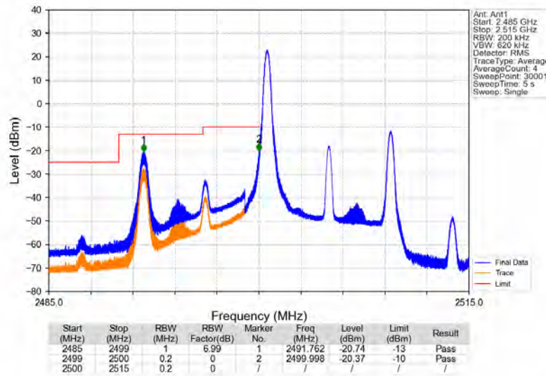
Band7_10MHz_16QAM_LCH_2505MHz_RB_1_0_NTNV
