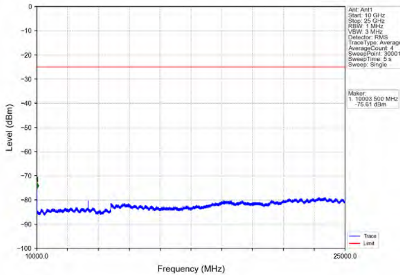
Band7_15MHz_QPSK_LCH_2507.5MHz_RB_1_0_NTNV
