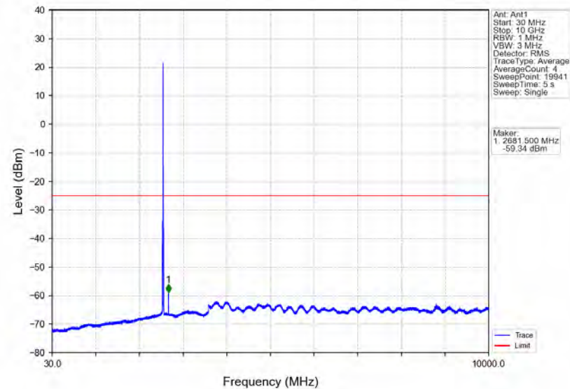
Band7_10MHz_16QAM_HCH_2565MHz_RB_1_0_NTNV
