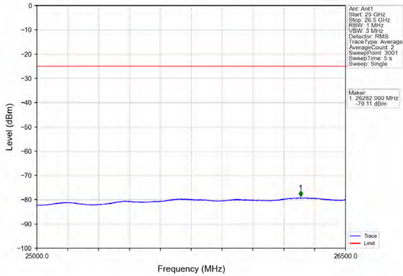
Band7_10MHz_16QAM_LCH_2505MHz_RB_50_0_NTNV
