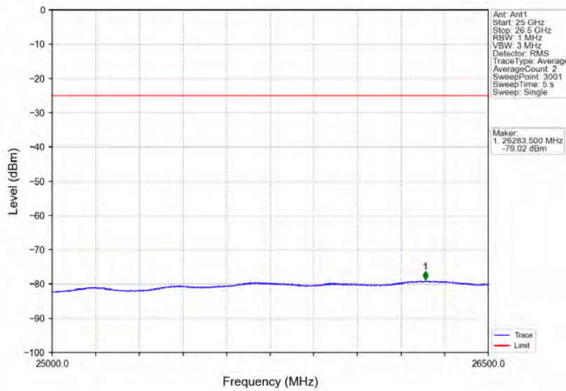
Band7_10MHz_16QAM_HCH_2565MHz_RB_1_0_NTNV
