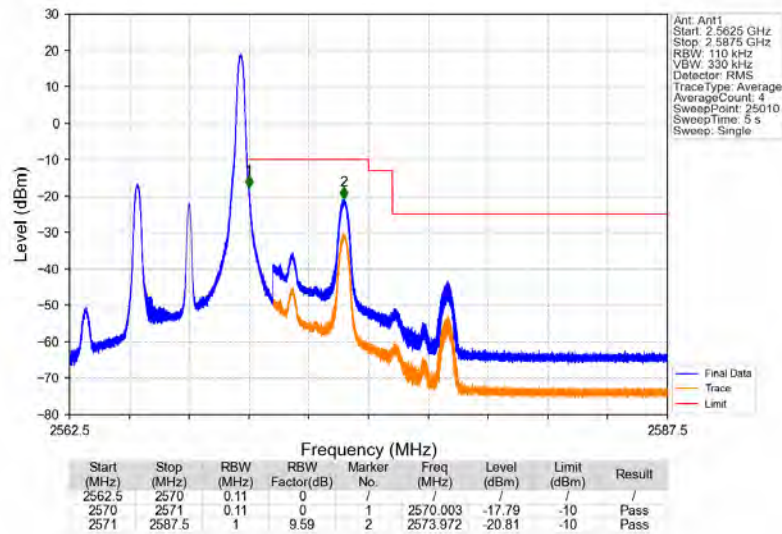
Band7_5MHz_16QAM_HCH_2567.5MHz_RB_1_24_NTNV
