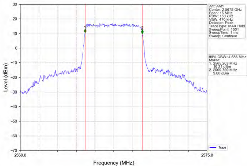
Band7_5MHz_16QAM_HCH_2567.5MHz_RB_25_0_NTNV
