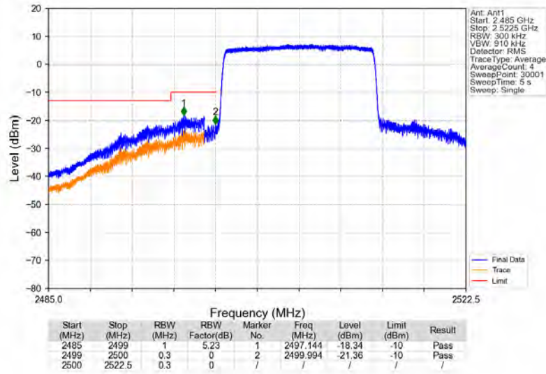
Band7_15MHz_16QAM_LCH_2507.5MHz_RB_75_0_NTNV
