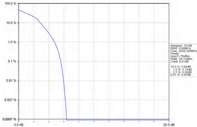
Band7_5MHz_16QAM_LCH_2502.5MHz_RB_25_0_NTNV
