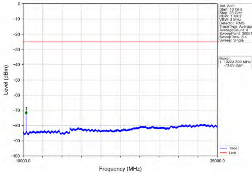
Band7_15MHz_QPSK_HCH_2562.5MHz_RB_1_0_NTNV
