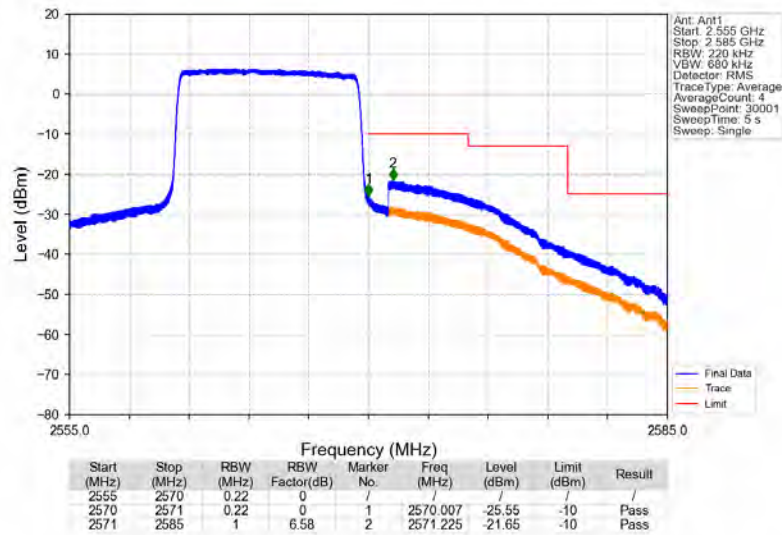
Band7_10MHz_16QAM_HCH_2565MHz_RB_50_0_NTV
