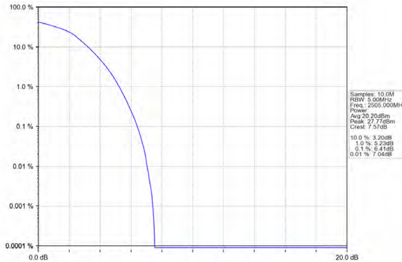
Band7_10MHz_16QAM_LCH_2505MHz_RB_50_0_NTNV
