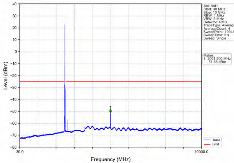
Band7_15MHz_16QAM_LCH_2507.5MHz_RB_1_0_NTNV
