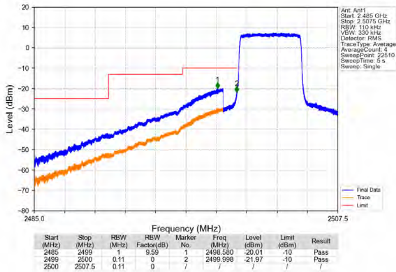
Band7_5MHz_16QAM_LCH_2502.5MHz_RB_25_0_NTNV
