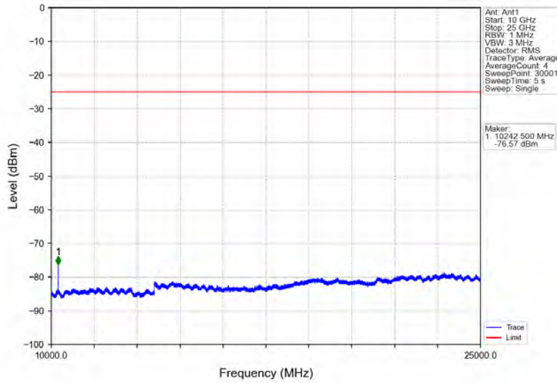
Band7_10MHz_16QAM_HCH_2565MHz_RB_1_0_NTNV
