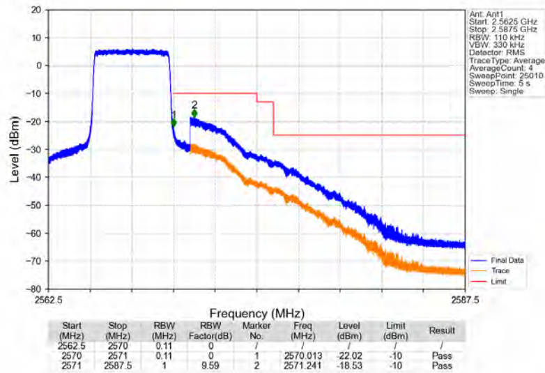
Band7_5MHz_16QAM_HCH_2567.5MHz_RB_25_0_NTNV
