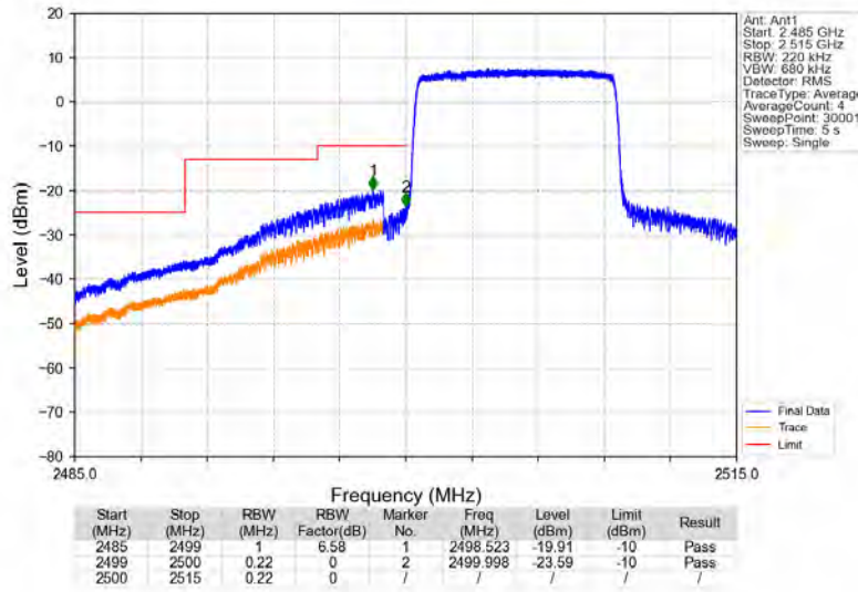
Band7_10MHz_16QAM_LCH_2505MHz_RB_50_0_NTNV
