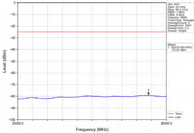
Band7_15MHz_16QAM_LCH_2507.5MHz_RB_75_0_NTNV
