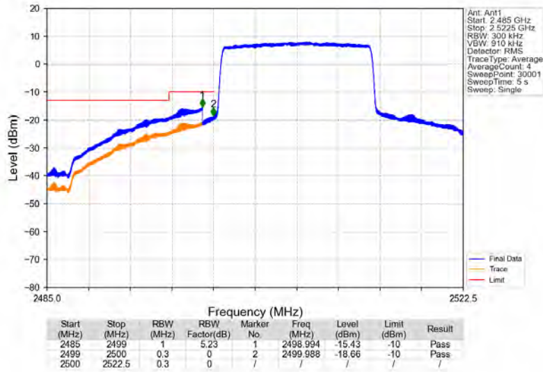
Band7_15MHz_QPSK_LCH_2507.5MHz_RB_75_0_NTNV
