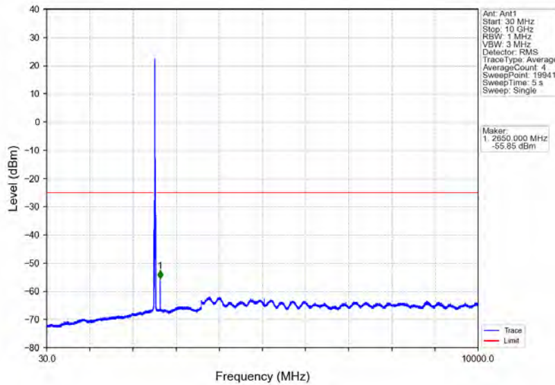
Band7_15MHz_16QAM_MCH_2535MHz_RB_1_0_NTNV
