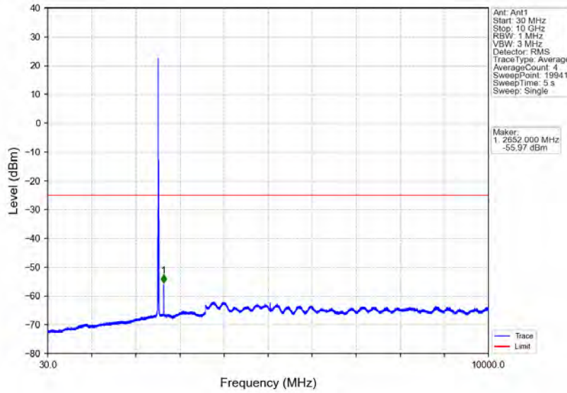
Band7_10MHz_16QAM_MCH_2535MHz_RB_1_0_NTNV
