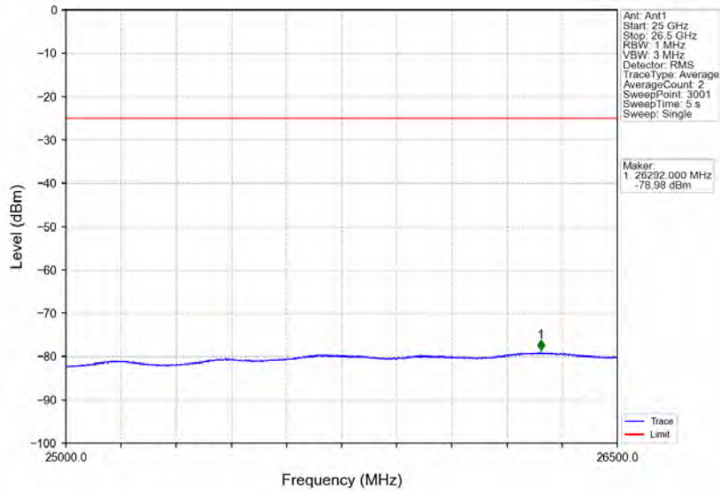
Band7_5MHz_16QAM_LCH_2502.5MHz_RB_25_0_NTNV
