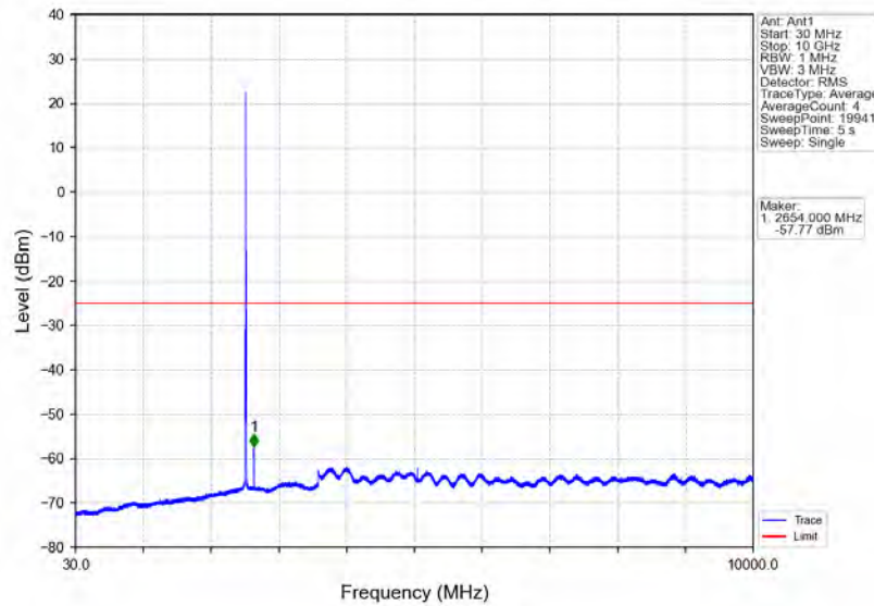
Band7_5MHz_16QAM_MCH_2535MHz_RB_1_0_NTNV
