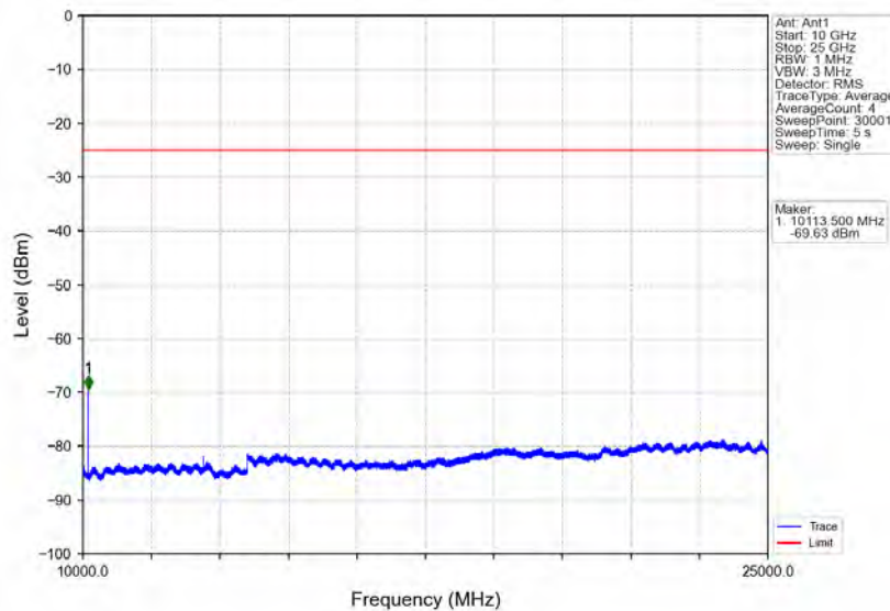
Band7_15MHz_16QAM_MCH_2535MHz_RB_1_0_NTNV
