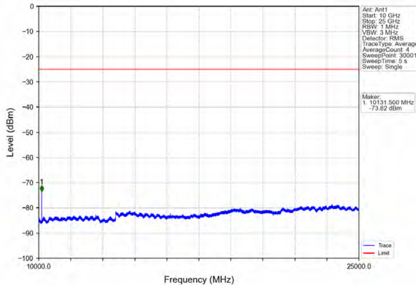
Band7_5MHz_16QAM_MCH_2535MHz_RB_1_0_NTNV
