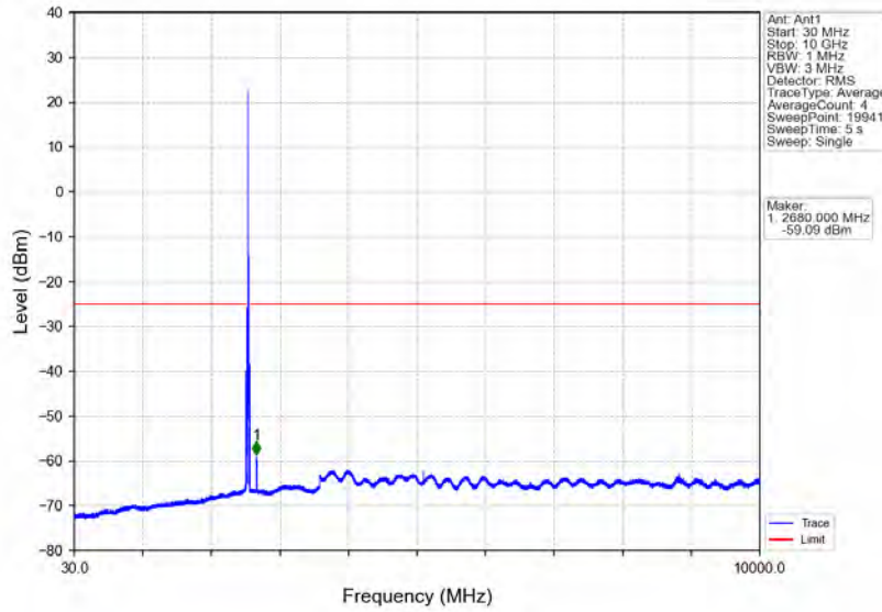
Band7_15MHz_QPSK_HCH_2562.5MHz_RB_1_0_NTNV
