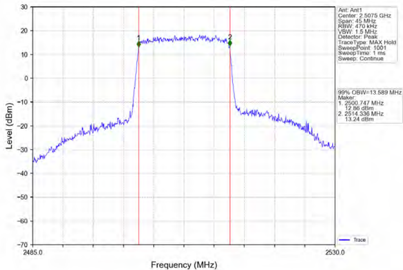
Band7_15MHz_16QAM_LCH_2507.5MHz_RB_75_0_NTNV
