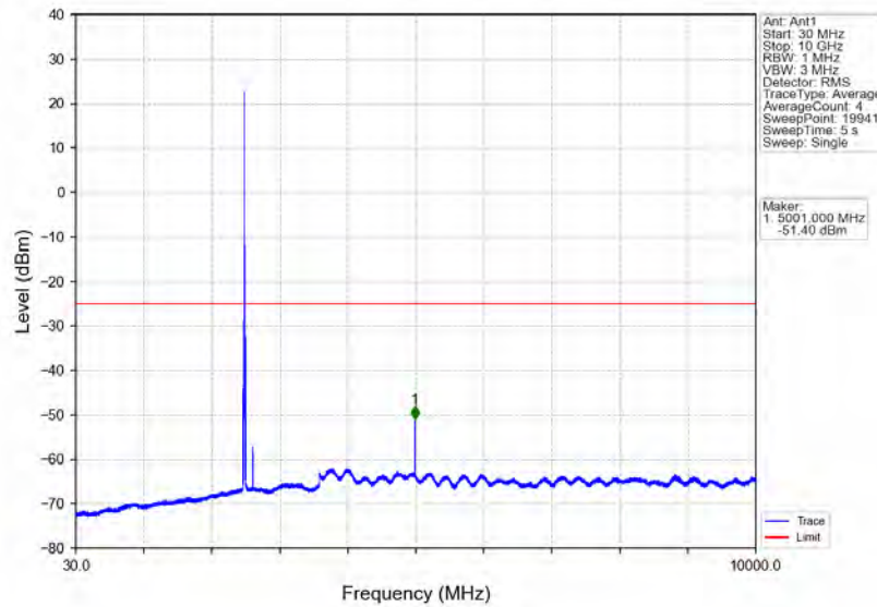
Band7_10MHz_16QAM_LCH_2505MHz_RB_1_0_NTNV
