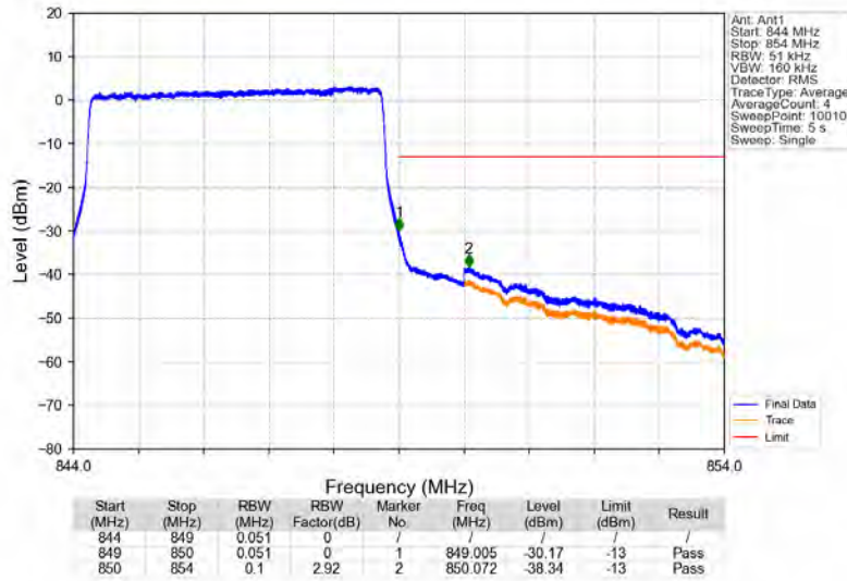
Band5_5MHz_QPSK_HCH_846.5MHz_RB_25_0_NTNV
