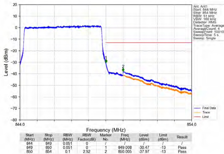
Band5_5MHz_16QAM_HCH_846.5MHz_RB_25_0_NTNV
