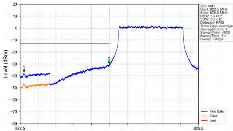
Band5_1.4MHz_16QAM_LCH_824.7MHz_RB_6_0_NTV
