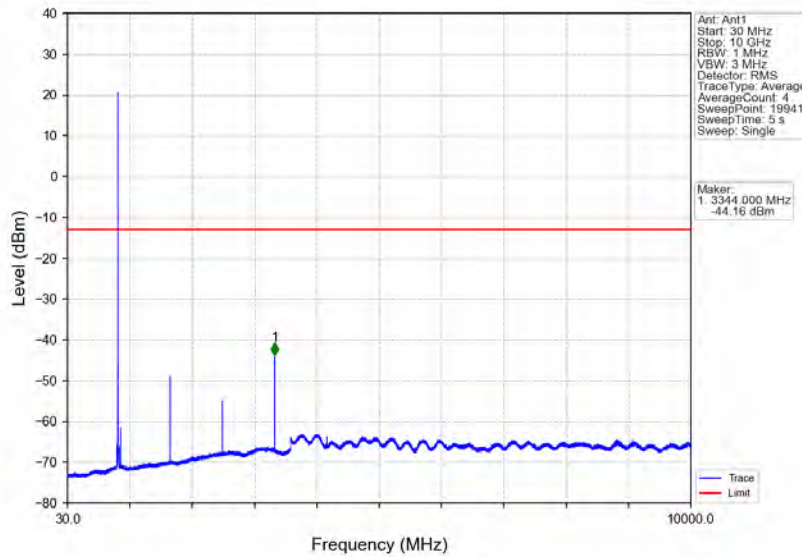
Band5_1.4MHz_16QAM_HCH_848.3MHz_RB_1_0_NTNV
