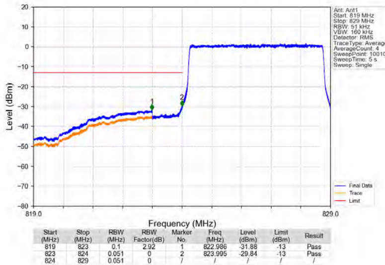
Band5_5MHz_16QAM_LCH_826.5MHz_RB_25_0_NTNV
