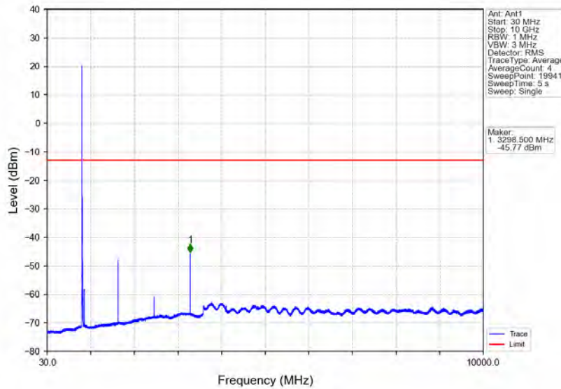
Band5_10MHz_16QAM_LCH_829MHz_RB_50_0_NTNV
