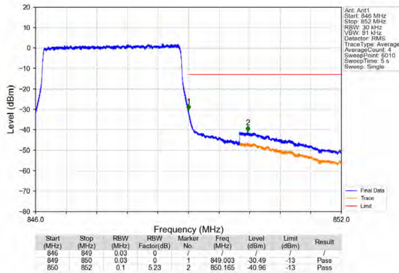
Band5_3MHz_16QAM_HCH_847.5MHz_RB_15_0_NTNV
