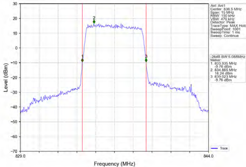
Band5_5MHz_QPSK_MCH_836.5MHz_RB_25_0_NTNV
