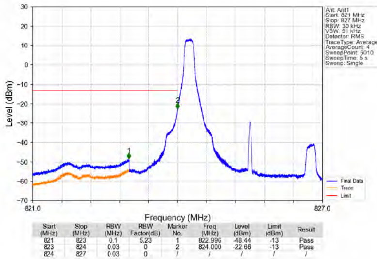
Band5_3MHz_16QAM_LCH_825.5MHz_RB_1_0_NTNV
