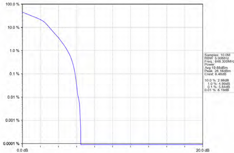
Band5_1.4MHz_16QAM_HCH_848.3MHz_RB_6_0_NTNV
