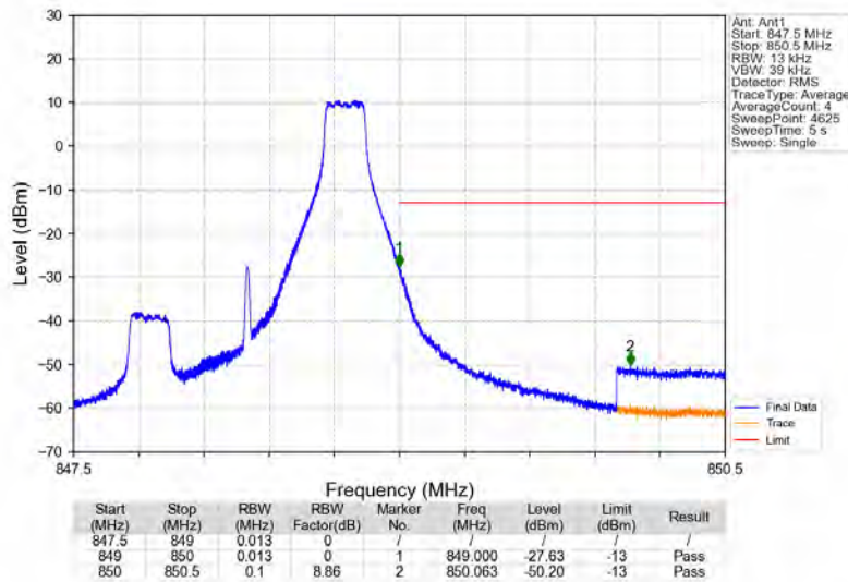
Band5_1.4MHz_16QAM_HCH_848.3MHz_RB_1_5_NTV
