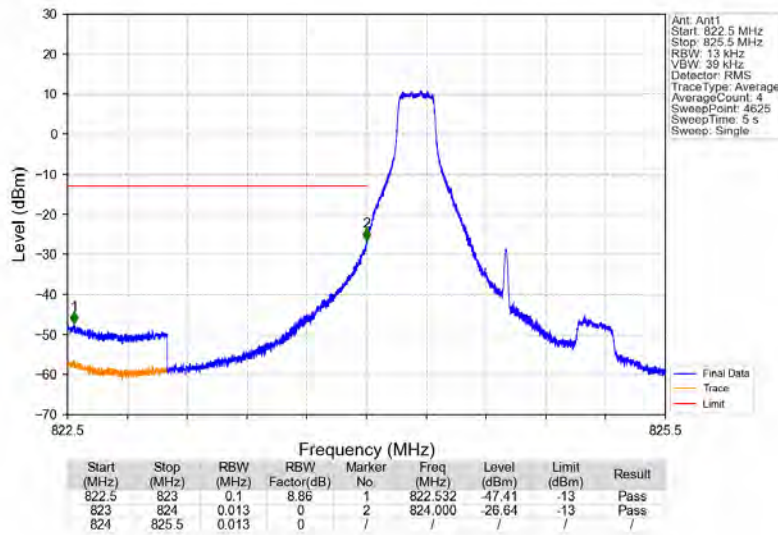
Band5_1.4MHz_16QAM_LCH_824.7MHz_RB_1_0_NTNV
