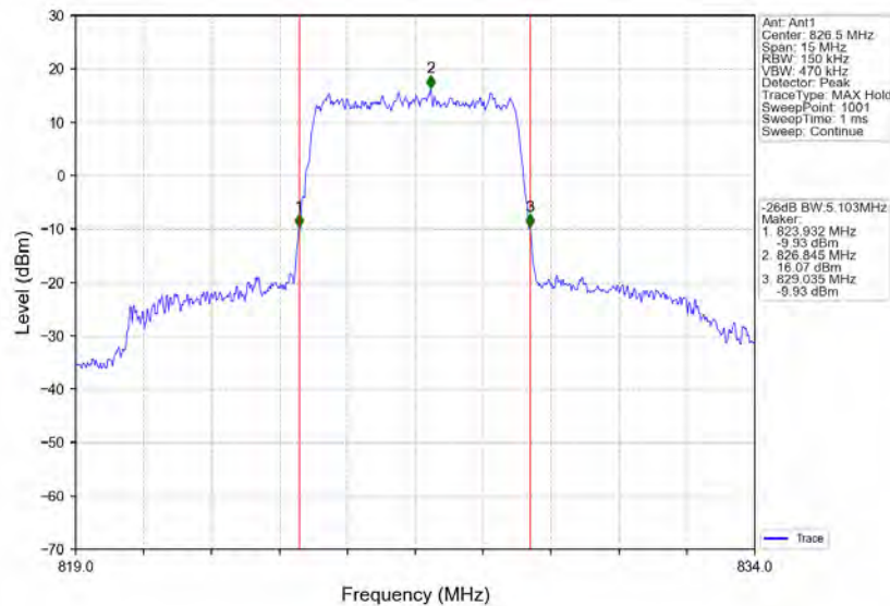
Band5_5MHz_16QAM_LCH_826.5MHz_RB_25_0_NTNV
