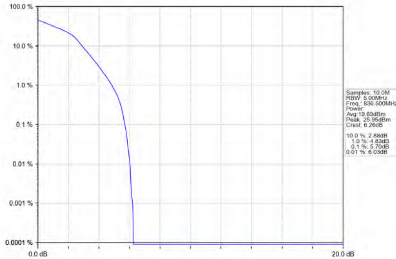
Band5_1.4MHz_16QAM_MCH_836.5MHz_RB_6_0_NTNV
