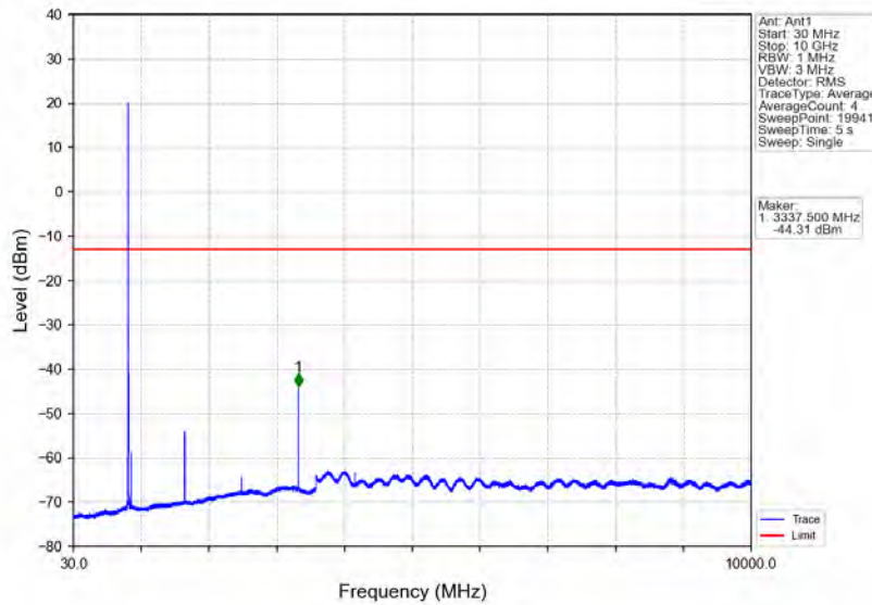
Band5_5MHz_16QAM_HCH_846.5MHz_RB_1_0_NTNV
