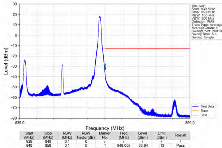
Band5_10MHz_16QAM_HCH_844MHz_RB_1_49_NTNV
