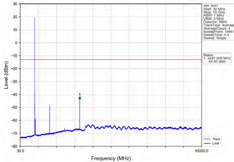
Band5_3MHz_16QAM_LCH_825.5MHz_RB_15_0_NTNV
