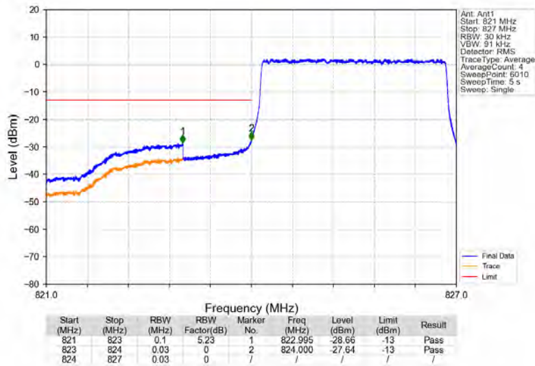
Band5_3MHz_QPSK_LCH_825.5MHz_RB_15_0_NTNV
