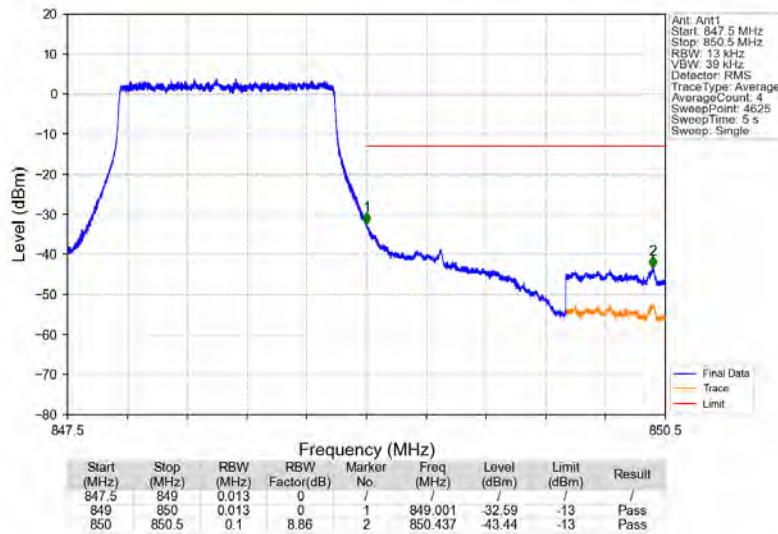
Band5_1.4MHz_QPSK_HCH_848.3MHz_RB_6_0_NTNV
