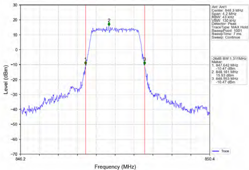
Band5_1.4MHz_16QAM_HCH_848.3MHz_RB_6_0_NTNV
