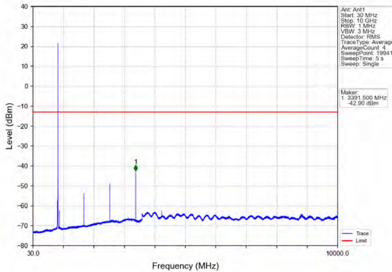
Band5_1.4MHz_QPSK_HCH_848.3MHz_RB_1_5_NTNV
