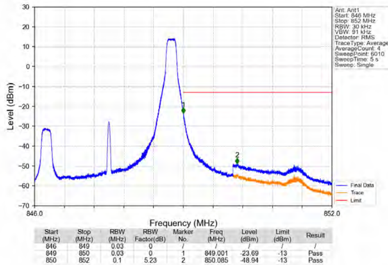
Band5_3MHz_16QAM_HCH_847.5MHz_RB_1_14_NTNV
