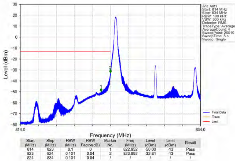
Band5_10MHz_16QAM_LCH_829MHz_RB_1_0_NTNV
