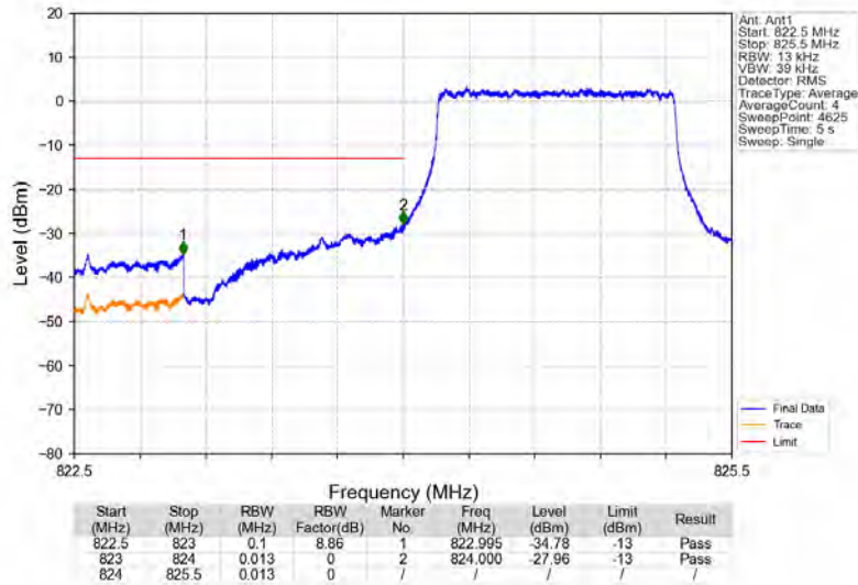
Band5_1.4MHz_QPSK_LCH_824.7MHz_RB_6_0_NTNV
