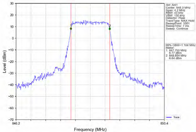
Band5_1.4MHz_16QAM_HCH_848.3MHz_RB_6_0_NTNV
