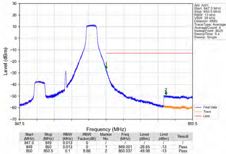
Band5_1.4MHz_QPSK_HCH_848.3MHz_RB_1_5_NTNV
