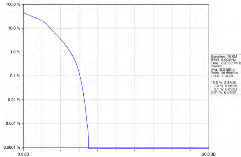
Band5_5MHz_16QAM_LCH_826.5MHz_RB_25_0_NTNV
