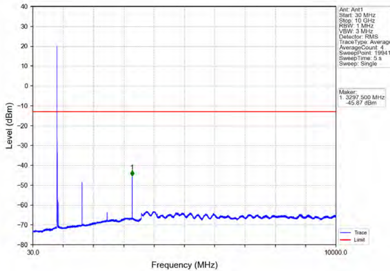
Band5_5MHz_16QAM_LCH_826.5MHz_RB_25_0_NTNV
