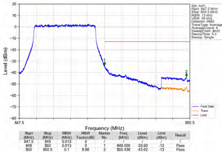
Band5_1.4MHz_16QAM_HCH_848.3MHz_RB_6_0_NTV
