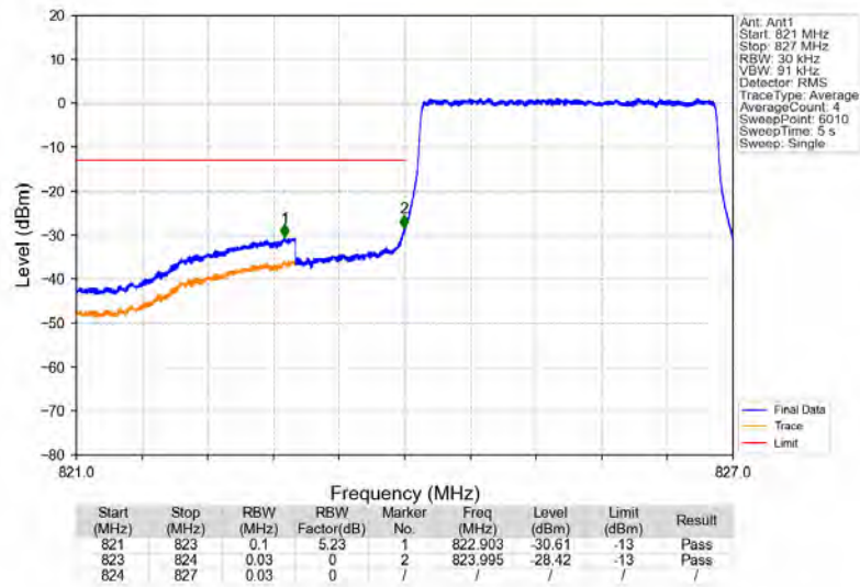
Band5_3MHz_16QAM_LCH_825.5MHz_RB_15_0_NTNV
