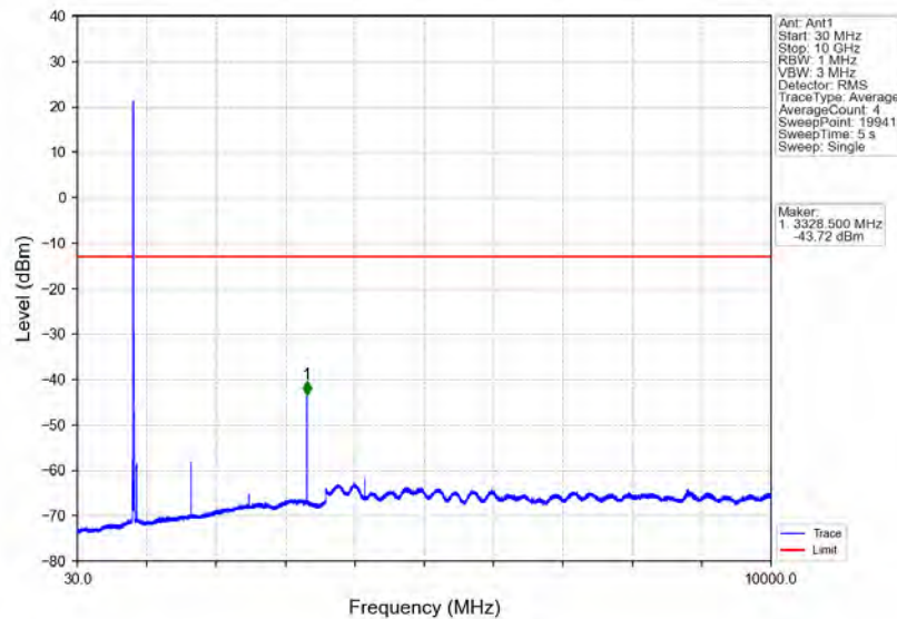
Band5_10MHz_QPSK_MCH_836.5MHz_RB_1_0_NTNV
