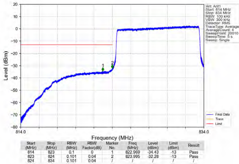
Band5_10MHz_16QAM_LCH_829MHz_RB_50_0_NTNV
