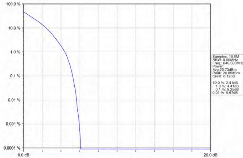
Band5_5MHz_QPSK_HCH_846.5MHz_RB_25_0_NTNV
