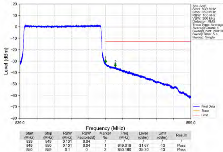
Band5_10MHz_16QAM_HCH_844MHz_RB_50_0_NTNV
