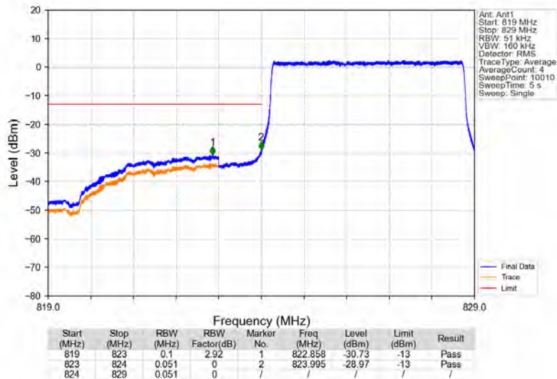
Band5_5MHz_QPSK_LCH_826.5MHz_RB_25_0_NTNV
