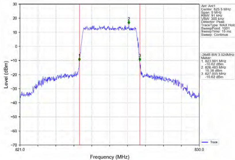
Band5_3MHz_16QAM_LCH_825.5MHz_RB_15_0_NTNV
