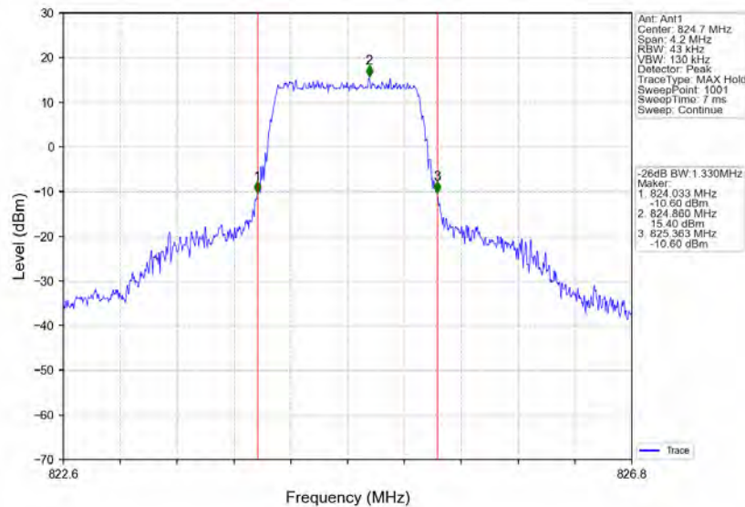
Band5_1.4MHz_16QAM_LCH_824.7MHz_RB_6_0_NTNV
