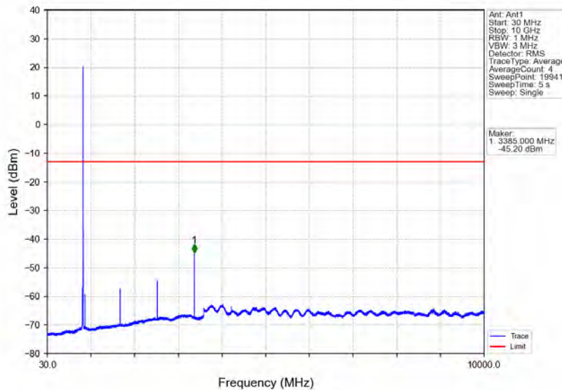
Band5_3MHz_16QAM_HCH_847.5MHz_RB_1_0_NTNV
