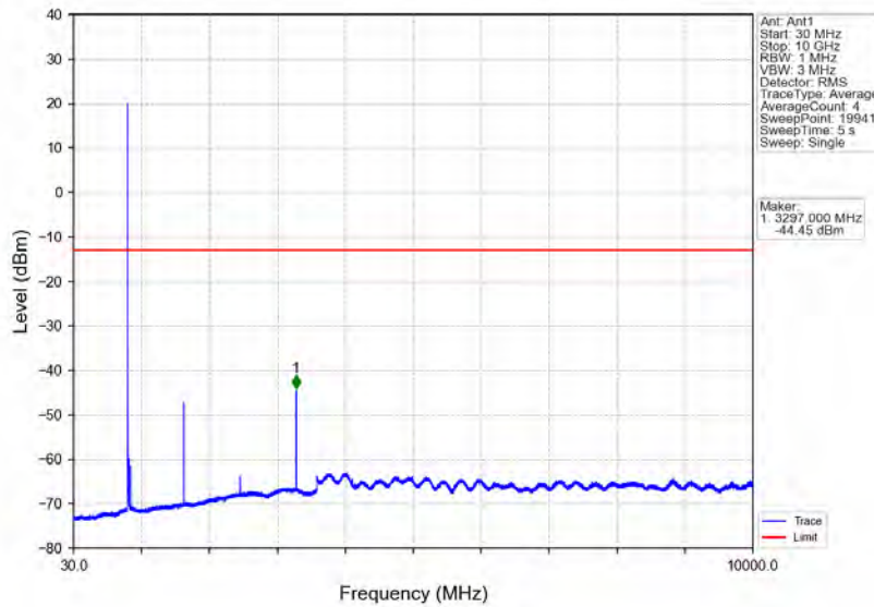
Band5_1.4MHz_16QAM_LCH_824.7MHz_RB_6_0_NTV
