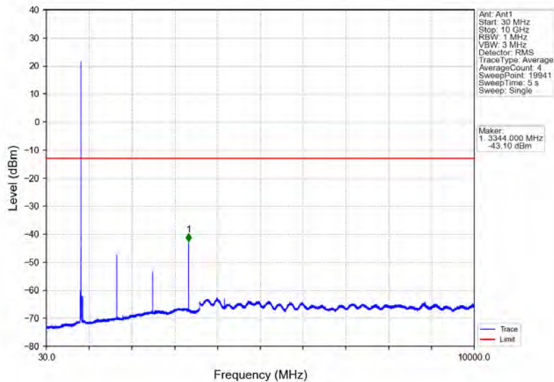
Band5_1.4MHz_QPSK_MCH_836.5MHz_RB_1_0_NTNV
