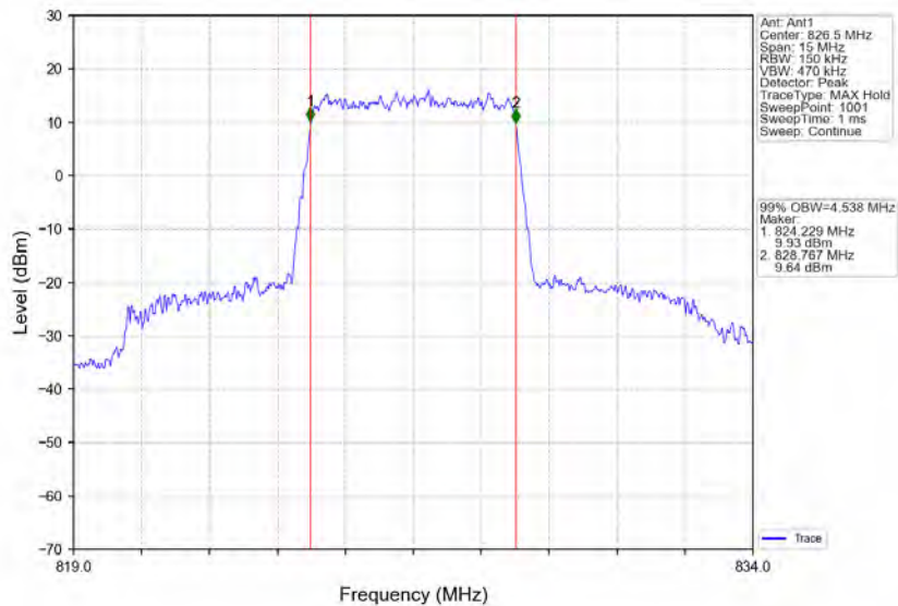
Band5_5MHz_16QAM_LCH_826.5MHz_RB_25_0_NTNV
