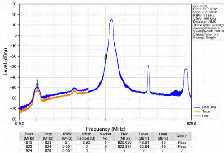
Band5_5MHz_16QAM_LCH_826.5MHz_RB_1_0_NTNV
