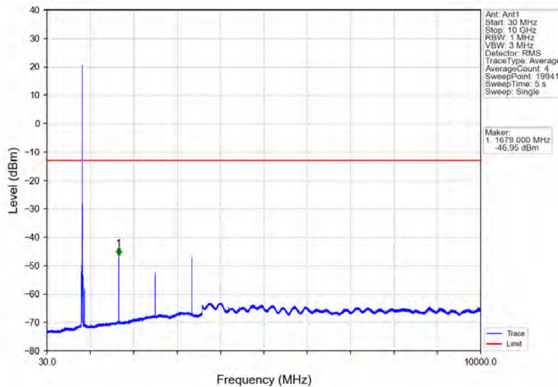
Band5_10MHz_16QAM_HCH_844MHz_RB_1_0_NTNV
