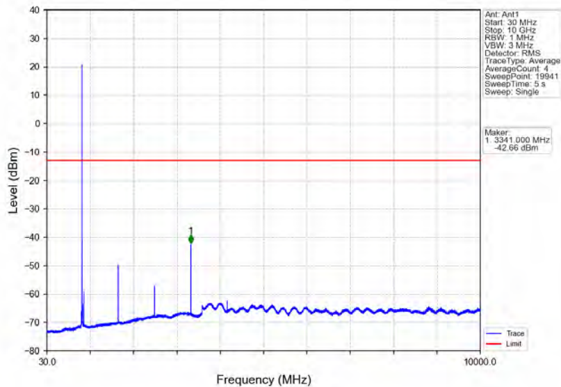
Band5_3MHz_QPSK_MCH_836.5MHz_RB_1_0_NTNV
