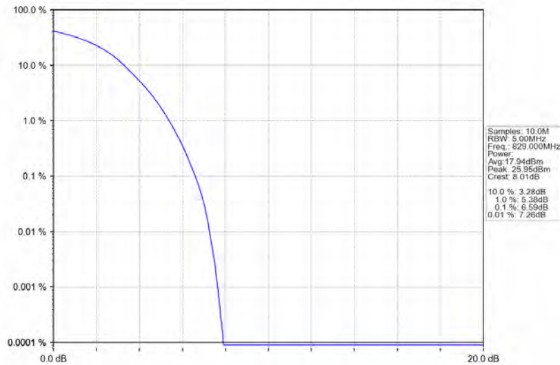
Band5_10MHz_16QAM_LCH_829MHz_RB_50_0_NTNV
