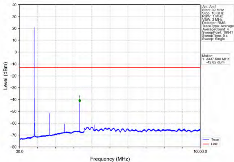
Band5_5MHz_QPSK_MCH_836.5MHz_RB_1_0_NTNV
