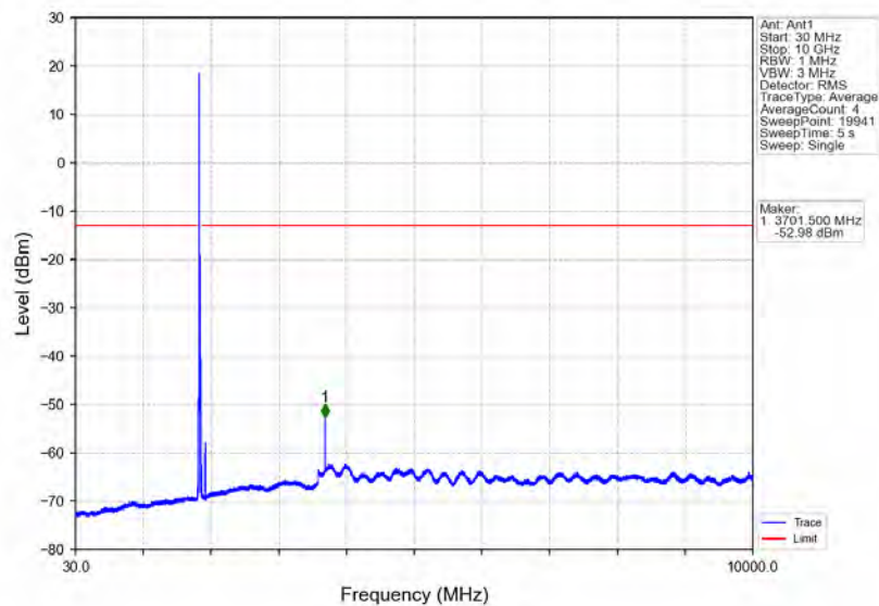
Band2_15MHz_16QAM_LCH_1857.5MHz_RB_1_0_NTNV
