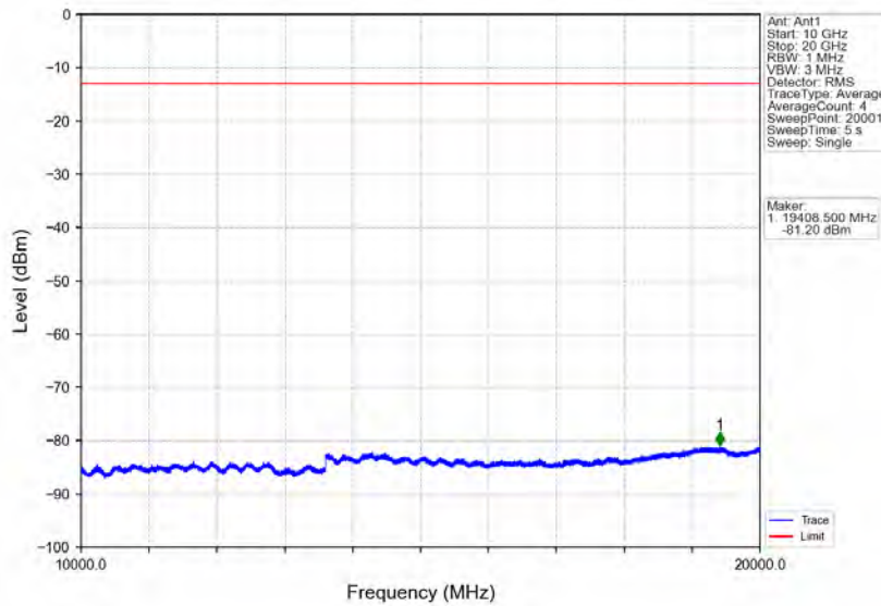
Band2_3MHz_16QAM_LCH_1851.5MHz_RB_15_0_NTNV
