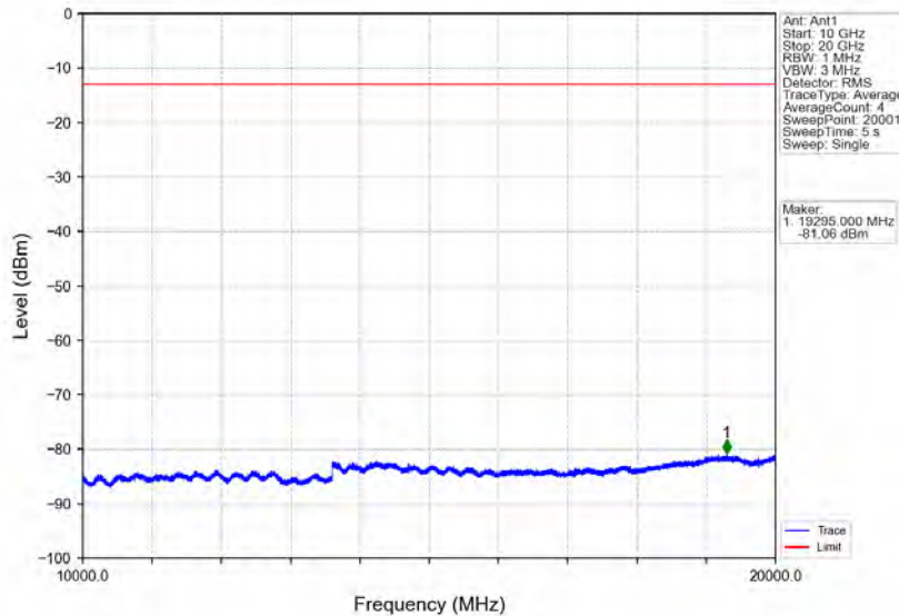
Band2_5MHz_QPSK_HCH_1907.5MHz_RB_1_0_NTNV
