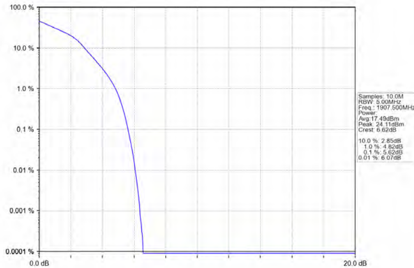
Band2_5MHz_16QAM_HCH_1907.5MHz_RB_25_0_NTNV
