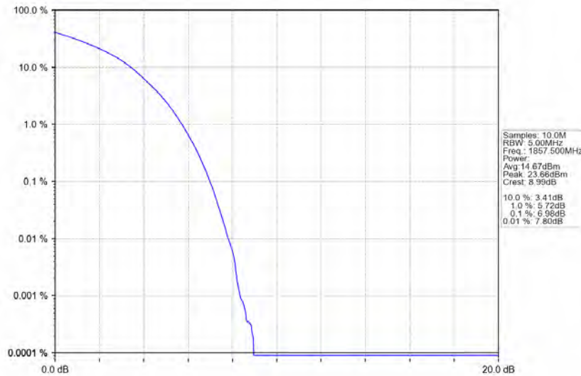
Band2_15MHz_16QAM_LCH_1857.5MHz_RB_75_0_NTNV
