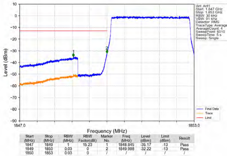
Band2_3MHz_16QAM_LCH_1851.5MHz_RB_15_0_NTNV
