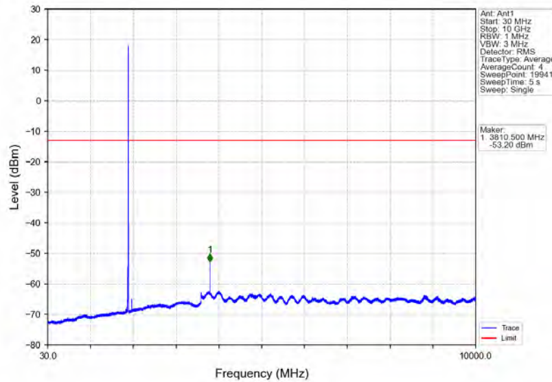
Band2_5MHz_16QAM_HCH_1907.5MHz_RB_1_0_NTNV
