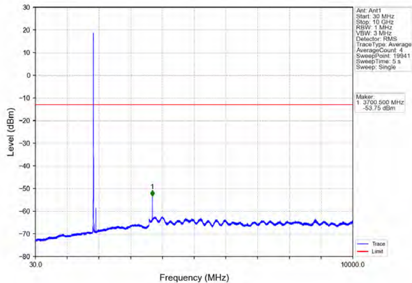
Band2_5MHz_16QAM_LCH_1852.5MHz_RB_1_0_NTNV
