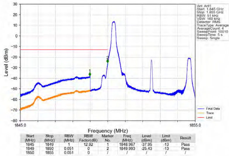
Band2_5MHz_16QAM_LCH_1852.5MHz_RB_1_0_NTNV
