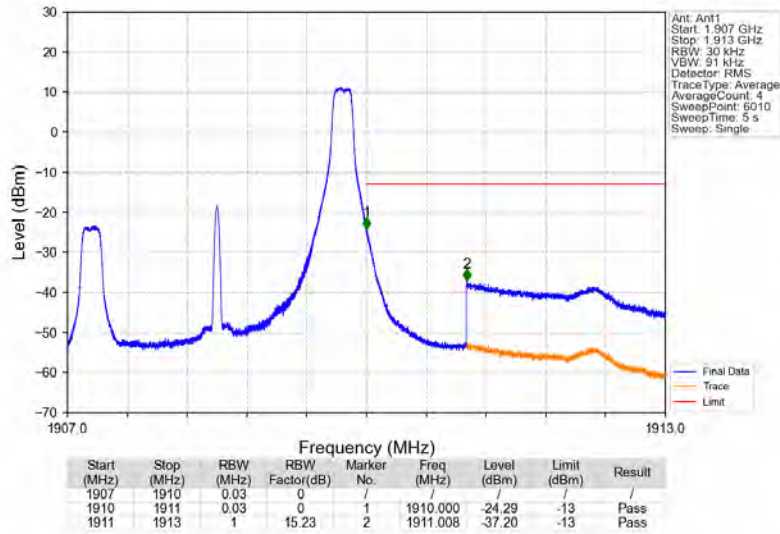
Band2_3MHz_16QAM_HCH_1908.5MHz_RB_1_14_NTNV
