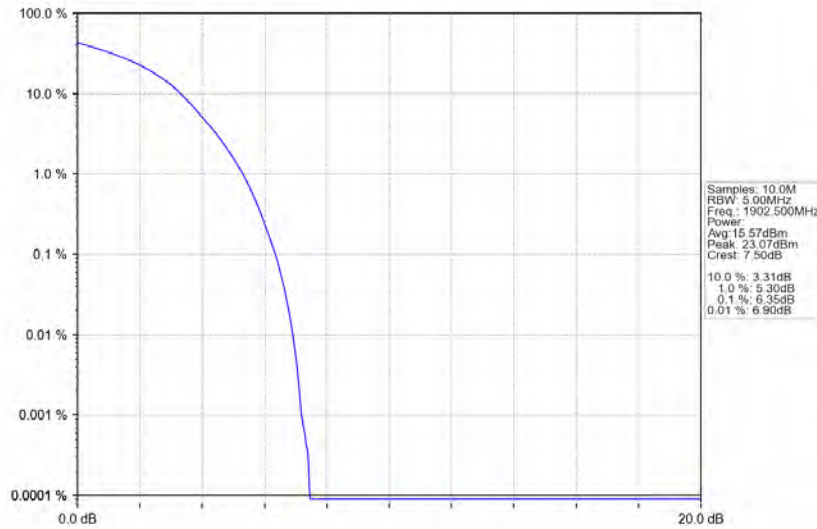
Band2_15MHz_QPSK_HCH_1902.5MHz_RB_75_0_NTNV
