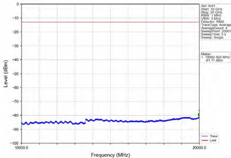
Band2_5MHz_16QAM_HCH_1907.5MHz_RB_1_0_NTNV
