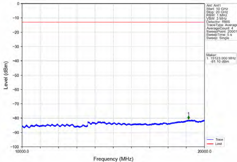
Band2_5MHz_16QAM_MCH_1880MHz_RB_1_0_NTNV
