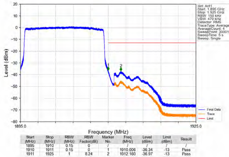
Band2_15MHz_QPSK_HCH_1902.5MHz_RB_75_0_NTNV
