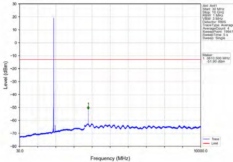
Band2_5MHz_QPSK_HCH_1907.5MHz_RB_1_0_NTNV
