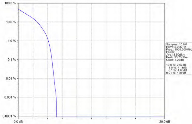
Band2_1.4MHz_QPSK_HCH_1909.3MHz_RB_6_0_NTNV
