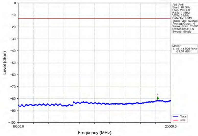
Band2_15MHz_16QAM_MCH_1880MHz_RB_1_0_NTNV
