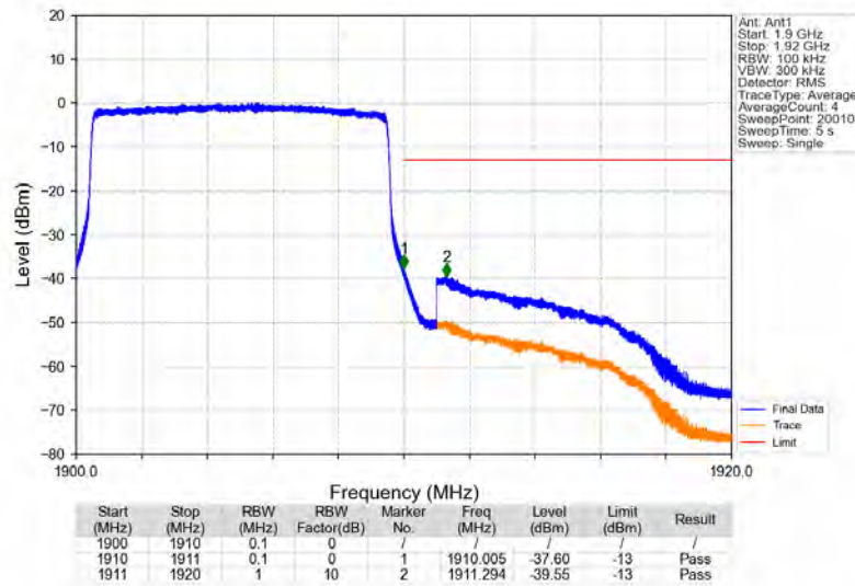
Band2_10MHz_16QAM_HCH_1905MHz_RB_50_0_NTV
