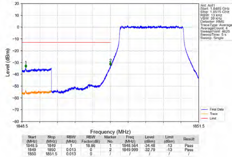
Band2_1.4MHz_QPSK_LCH_1850.7MHz_RB_6_0_NTNV
