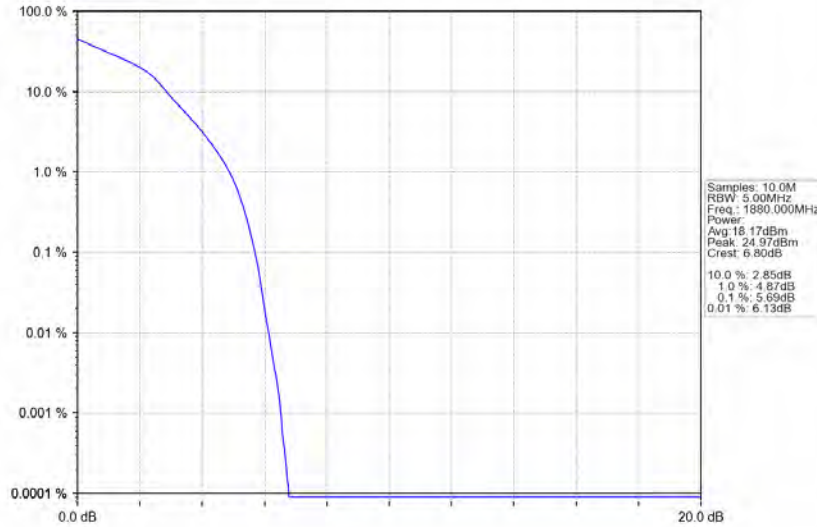
Band2_5MHz_16QAM_MCH_1880MHz_RB_25_0_NTNV
