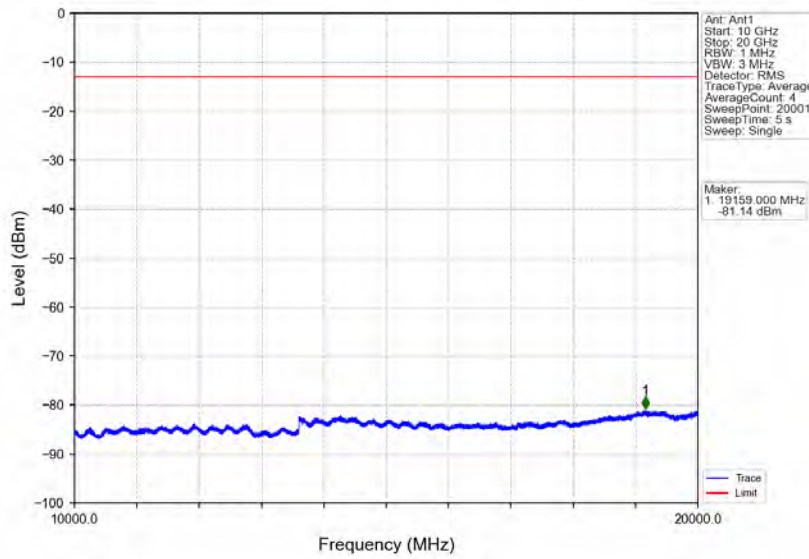
Band2_5MHz_QPSK_LCH_1852.5MHz_RB_25_0_NTNV
