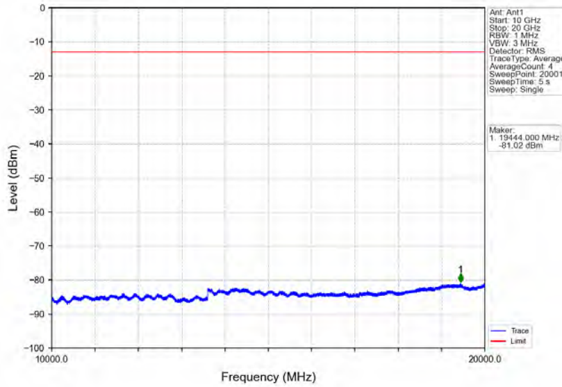
Band2_1.4MHz_QPSK_LCH_1850.7MHz_RB_6_0_NTNV
