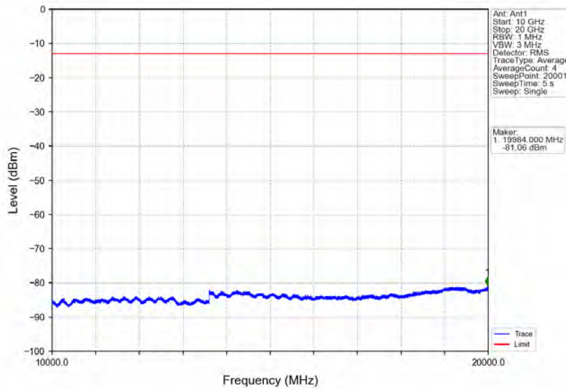
Band2_15MHz_16QAM_LCH_1857.5MHz_RB_75_0_NTNV
