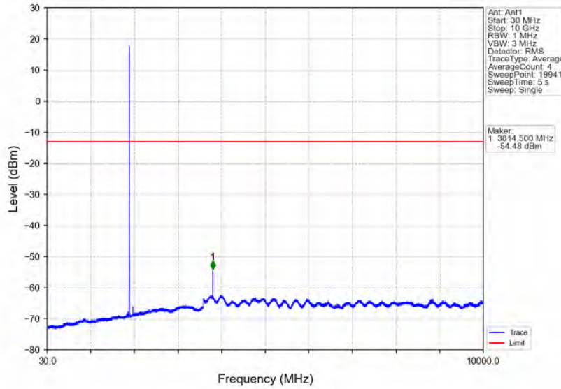
Band2_3MHz_16QAM_HCH_1908.5MHz_RB_1_0_NTNV
