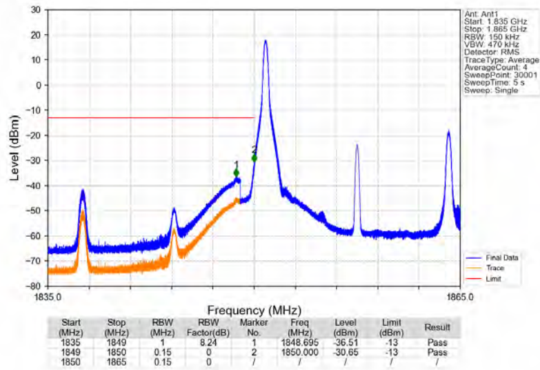
Band2_15MHz_16QAM_LCH_1857.5MHz_RB_1_0_NTNV
