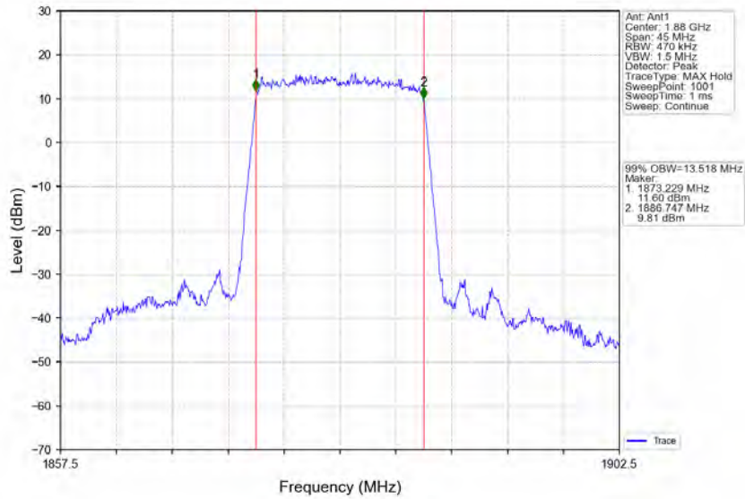
Band2_15MHz_QPSK_MCH_1880MHz_RB_75_0_NTNV
