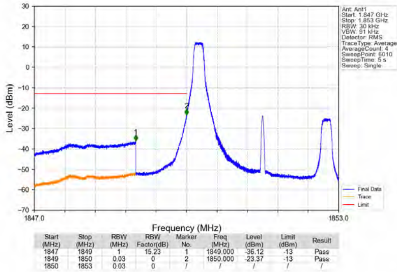
Band2_3MHz_16QAM_LCH_1851.5MHz_RB_1_0_NTNV
