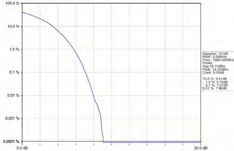
Band2_15MHz_16QAM_MCH_1880MHz_RB_75_0_NTNV
