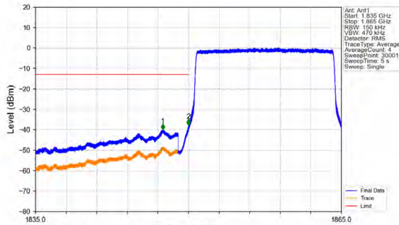
Band2_15MHz_16QAM_LCH_1857.5MHz_RB_75_0_NTNV
