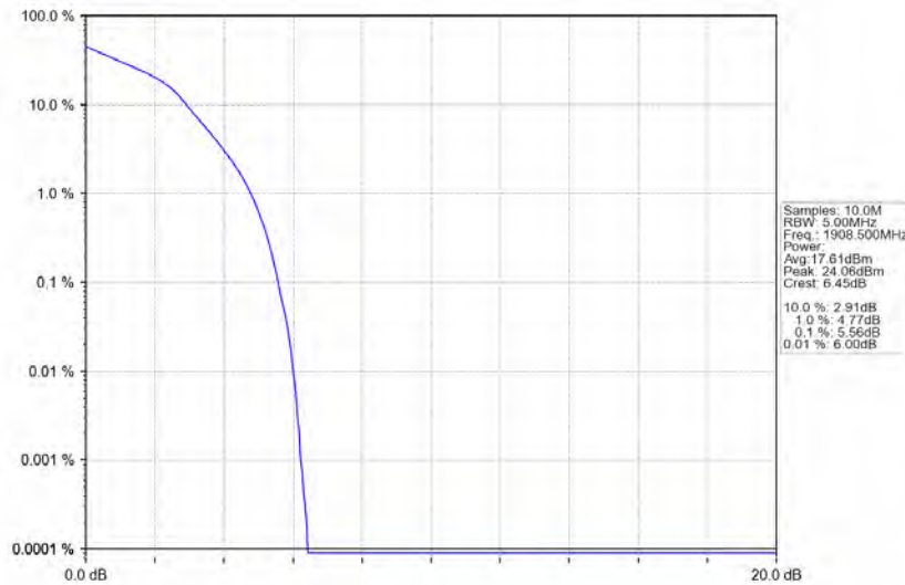
Band2_3MHz_16QAM_HCH_1908.5MHz_RB_15_0_NTNV
