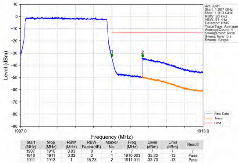
Band2_3MHz_16QAM_HCH_1908.5MHz_RB_15_0_NTNV
