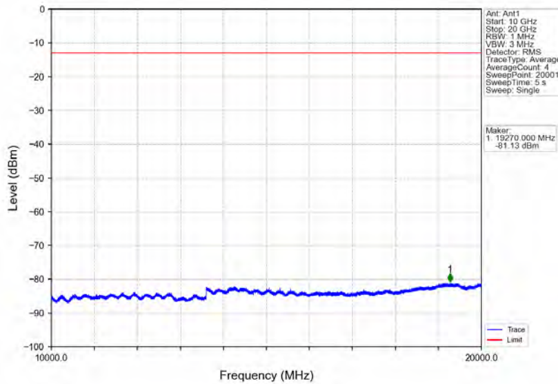
Band2_3MHz_QPSK_LCH_1851.5MHz_RB_15_0_NTNV
