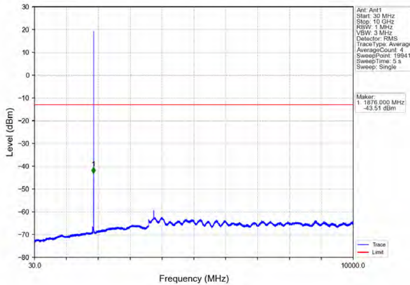
Band2_1.4MHz_16QAM_MCH_1880MHz_RB_1_0_NTNV
