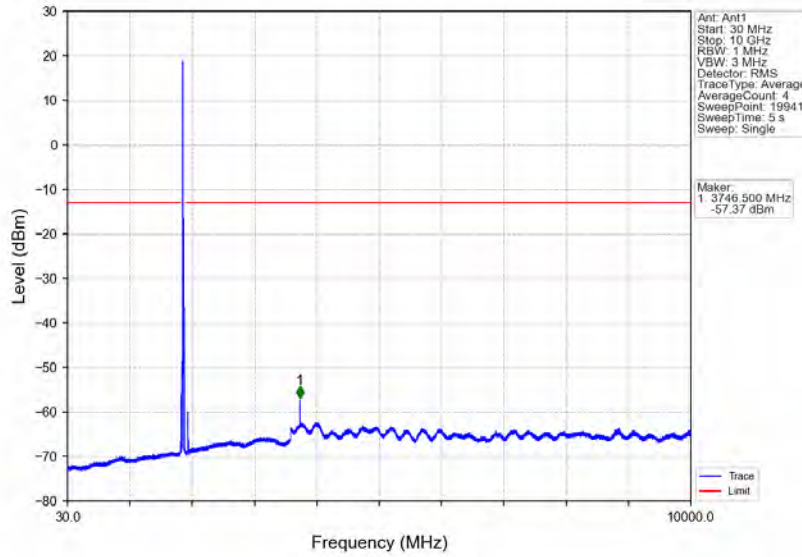
Band2_15MHz_16QAM_MCH_1880MHz_RB_1_0_NTNV
