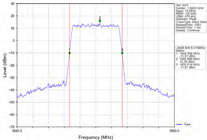
Band2_5MHz_16QAM_LCH_1852.5MHz_RB_25_0_NTNV
