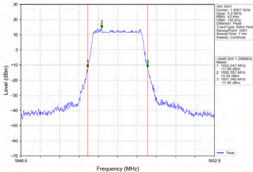
Band2_1.4MHz_16QAM_LCH_1850.7MHz_RB_6_0_NTNV
