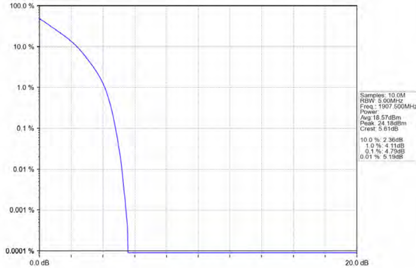
Band2_5MHz_QPSK_HCH_1907.5MHz_RB_25_0_NTNV
