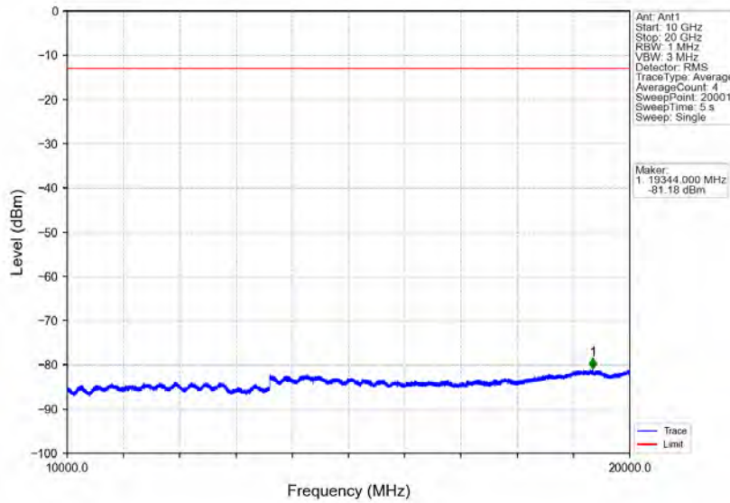
Band2_3MHz_16QAM_HCH_1908.5MHz_RB_1_0_NTNV
