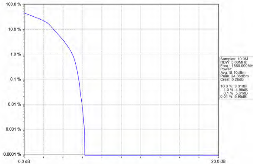
Band2_1.4MHz_16QAM_MCH_1880MHz_RB_6_0_NTNV
