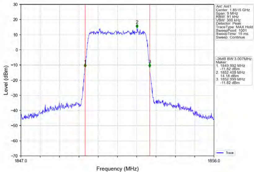
Band2_3MHz_16QAM_LCH_1851.5MHz_RB_15_0_NTNV
