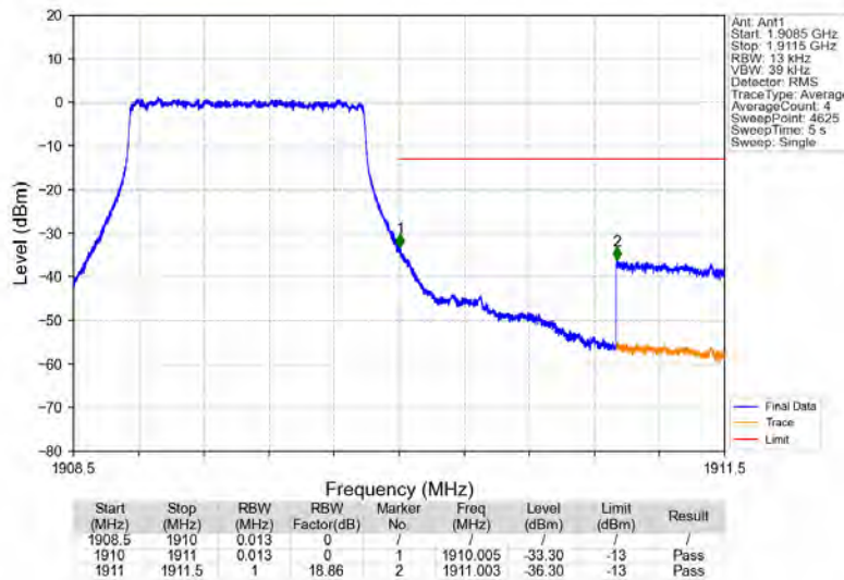
Band2_1.4MHz_QPSK_HCH_1909.3MHz_RB_6_0_NTV
