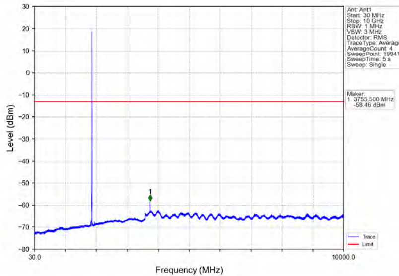
Band2_5MHz_16QAM_MCH_1880MHz_RB_1_0_NTNV
