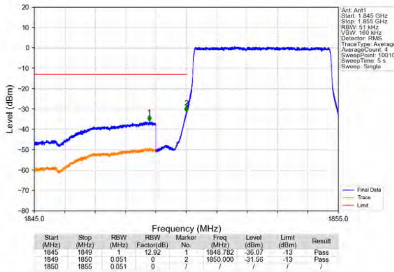
Band2_5MHz_QPSK_LCH_1852.5MHz_RB_25_0_NTNV
