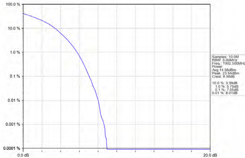
Band2_15MHz_16QAM_HCH_1902.5MHz_RB_75_0_NTNV
