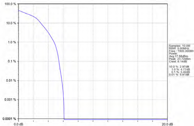
Band2_1.4MHz_16QAM_HCH_1909.3MHz_RB_6_0_NTNV
