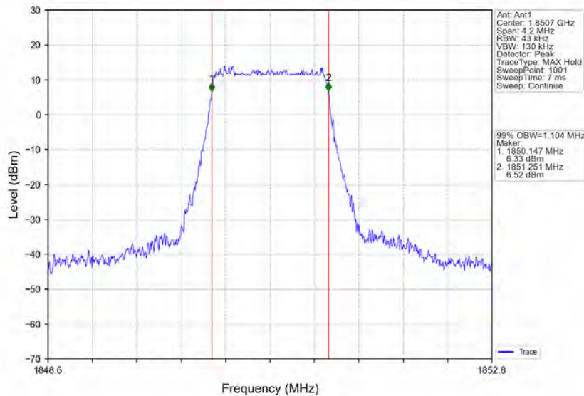
Band2_1.4MHz_16QAM_LCH_1850.7MHz_RB_6_0_NTNV
