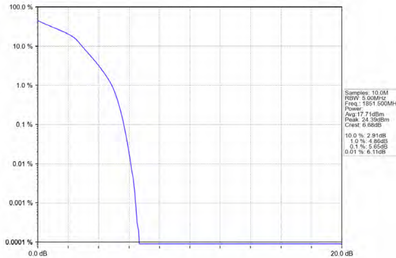
Band2_3MHz_16QAM_LCH_1851.5MHz_RB_15_0_NTNV
