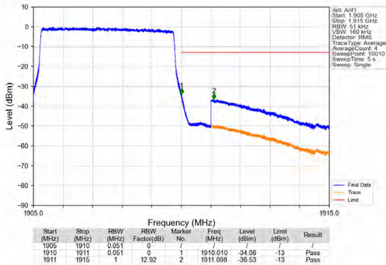
Band2_5MHz_16QAM_HCH_1907.5MHz_RB_25_0_NTNV
