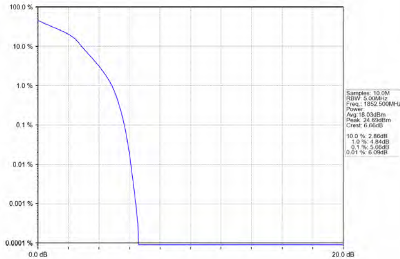
Band2_5MHz_16QAM_LCH_1852.5MHz_RB_25_0_NTNV
