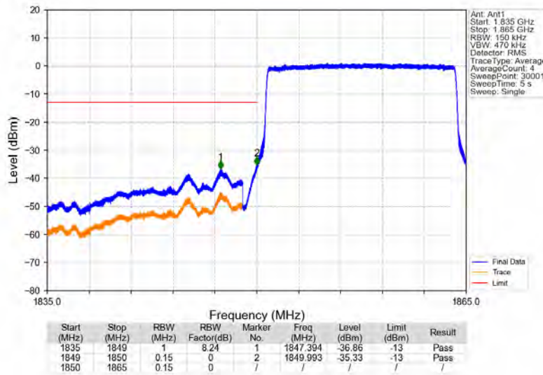
Band2_15MHz_QPSK_LCH_1857.5MHz_RB_75_0_NTNV
