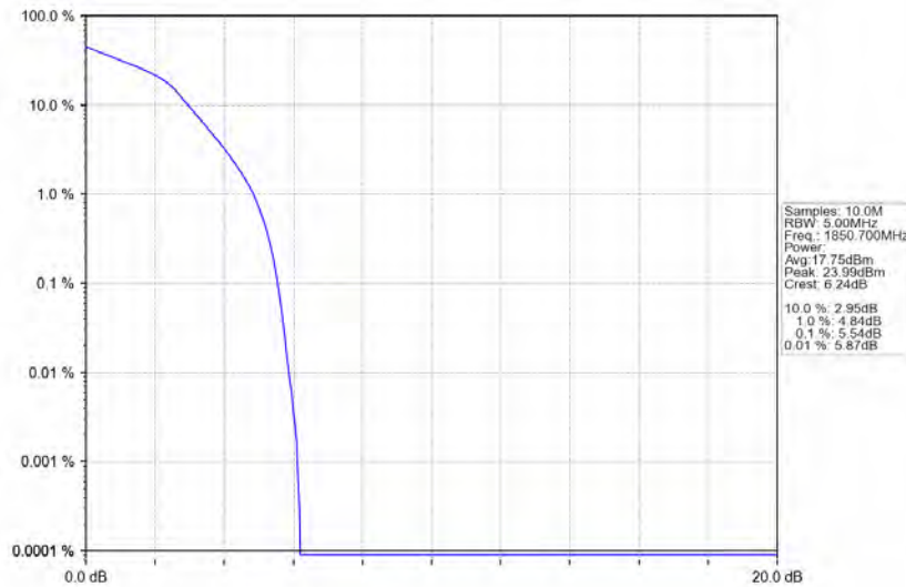
Band2_1.4MHz_16QAM_LCH_1850.7MHz_RB_6_0_NTNV
