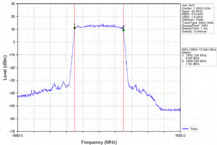
Band2_15MHz_16QAM_HCH_1902.5MHz_RB_75_0_NTNV
