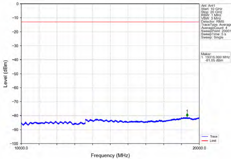
Band2_15MHz_QPSK_LCH_1857.5MHz_RB_75_0_NTNV
