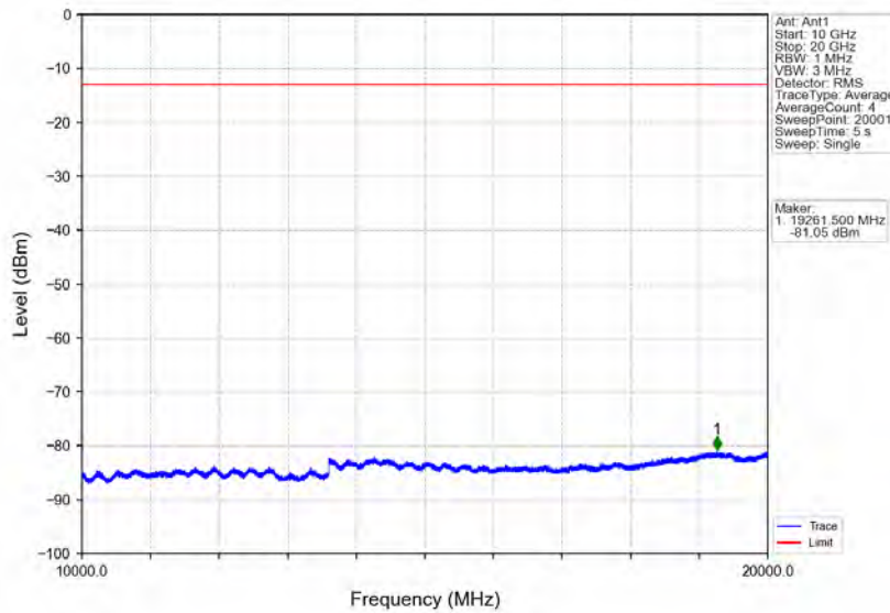
Band2_5MHz_16QAM_LCH_1852.5MHz_RB_25_0_NTNV
