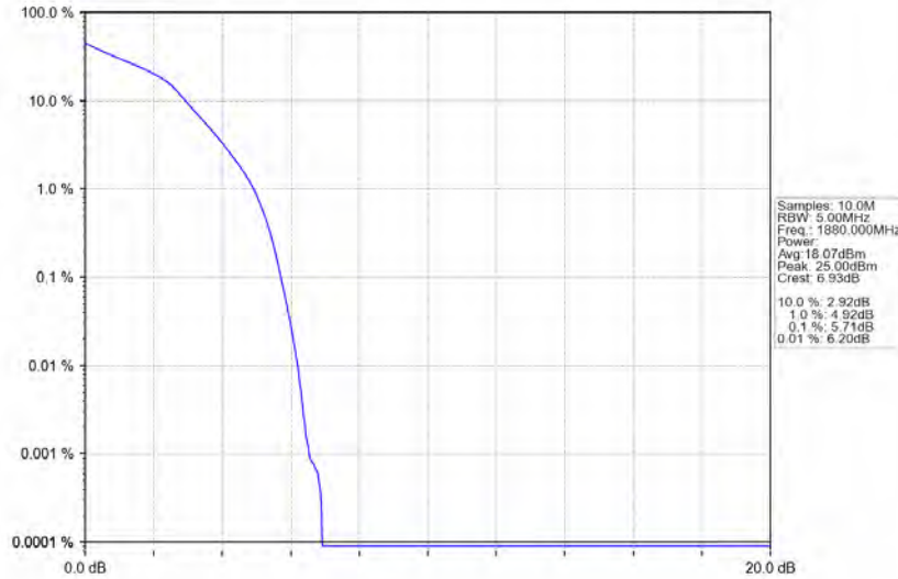
Band2_3MHz_16QAM_MCH_1880MHz_RB_15_0_NTNV
