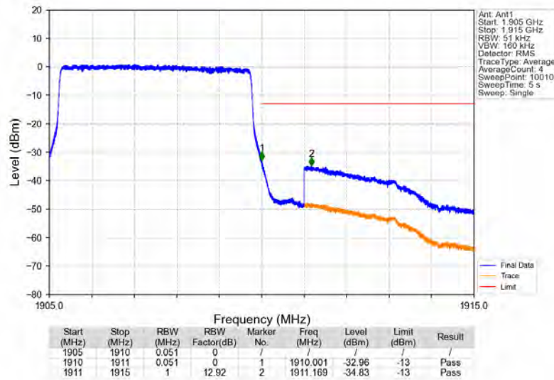
Band2_5MHz_QPSK_HCH_1907.5MHz_RB_25_0_NTNV
