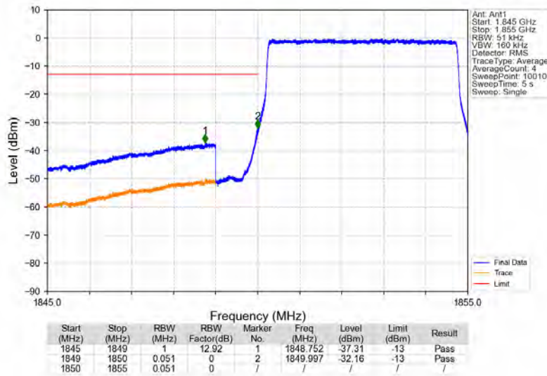
Band2_5MHz_16QAM_LCH_1852.5MHz_RB_25_0_NTNV
