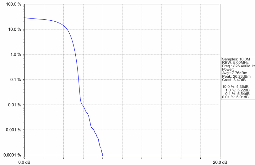
Band5_HSUPA_LCH_826.4MHz_Subtest 1_NTNV
