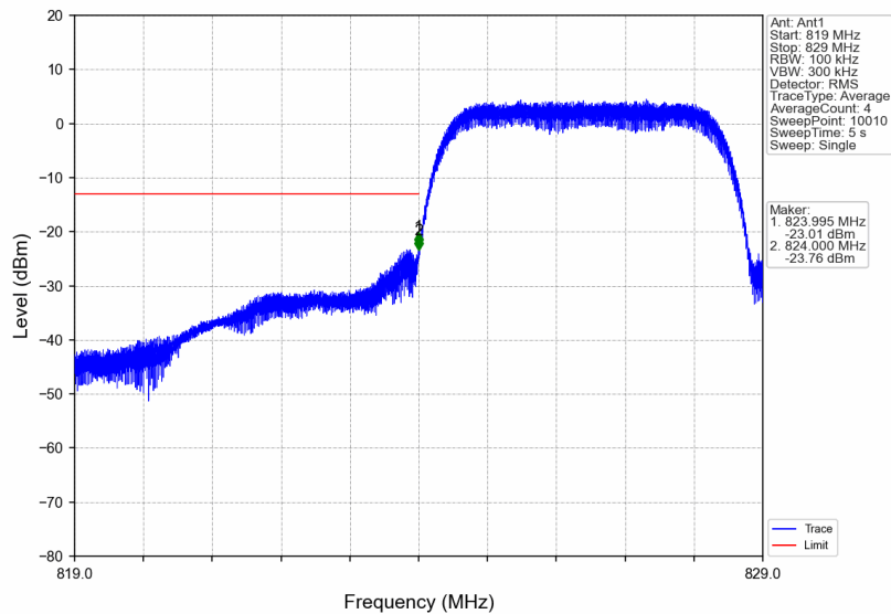
Band5_HSDPA_LCH_826.4MHz_Subtest 1_NTNV
