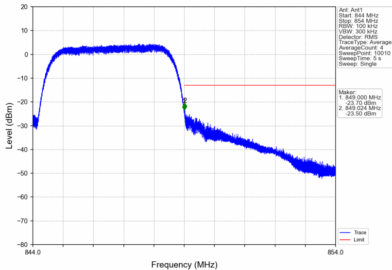
Band5_HSUPA_HCH_846.6MHz_Subtest 1_NTNV
