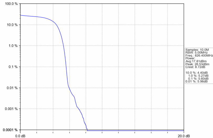
Band5_HSDPA_LCH_826.4MHz_Subtest 1_NTNV
