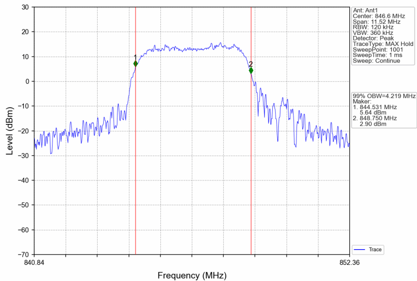
Band5_HSDPA_HCH_846.6MHz_Subtest 1_NTNV
