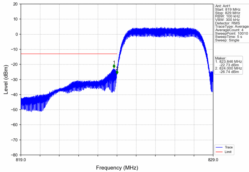
Band5_HSUPA_LCH_826.4MHz_Subtest 1_NTNV
