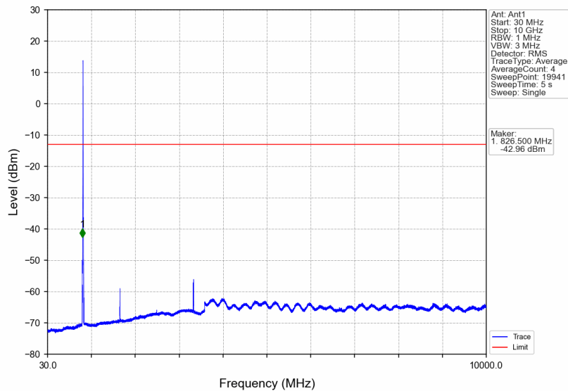
Band5_HSDPA_MCH_836.6MHz_Subtest 1_NTNV
