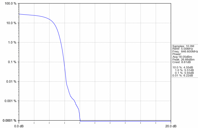
Band5_HSDPA_HCH_846.6MHz_Subtest 1_NTNV
