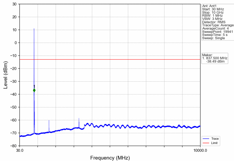
Band5_HSUPA_LCH_826.4MHz_Subtest 1_NTNV
