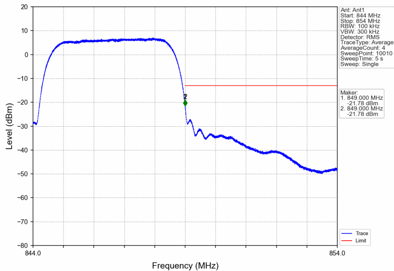
Band5_RMC_HCH_846.6MHz_12.2kbps RMC_NTNV
