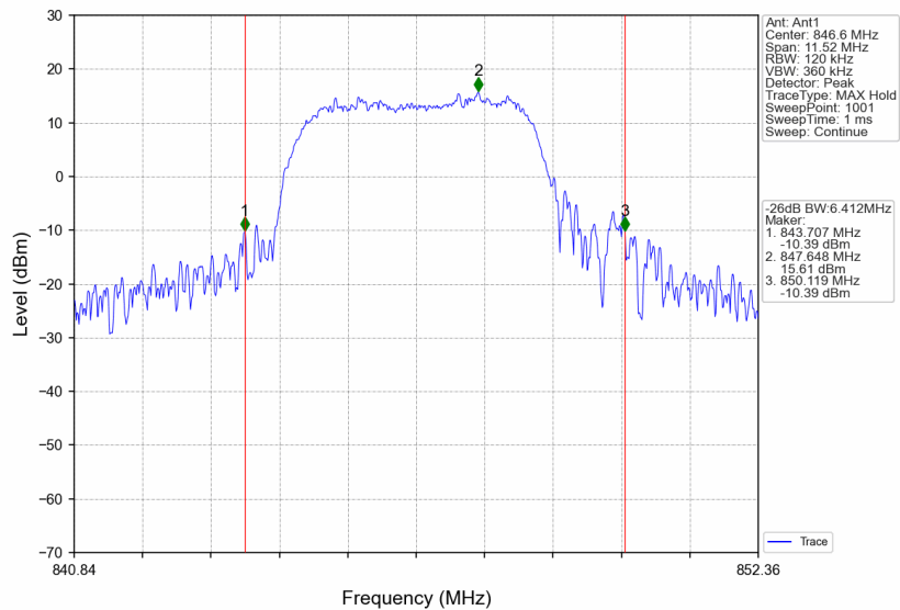
Band5_HSDPA_HCH_846.6MHz_Subtest 1_NTNV
