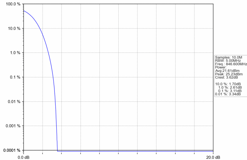
Band5_RMC_HCH_846.6MHz_12.2kbps RMC_NTNV
