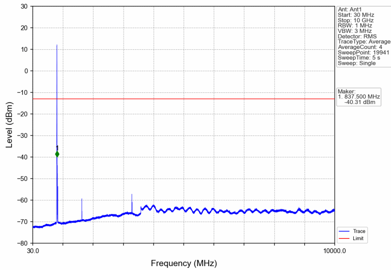
Band5_HSDPA_MCH_836.6MHz_Subtest 1_NTNV
