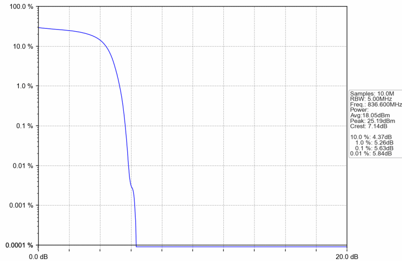
Band5_HSDPA_MCH_836.6MHz_Subtest 1_NTNV
