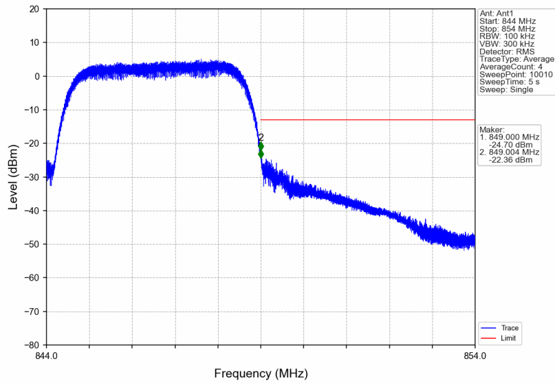
Band5_HSDPA_HCH_846.6MHz_Subtest 1_NTNV
