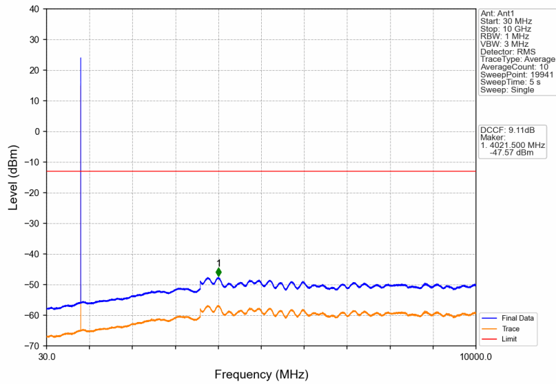
GSM850_EGPRS_MCH_836.6MHz_1 TX Slot_NTNV
