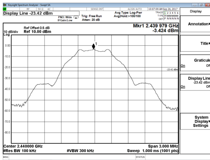
Channel 19 / 2440 MHz
