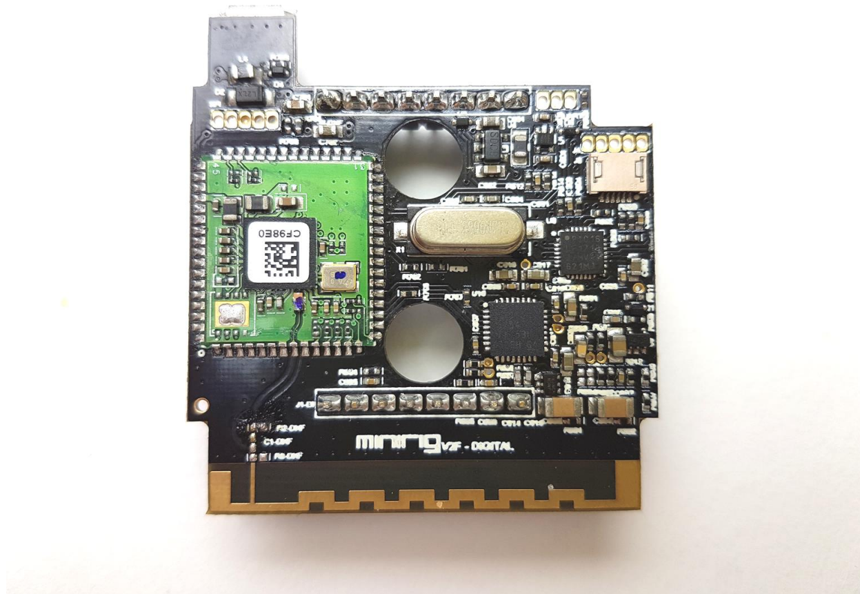
Digital board top
