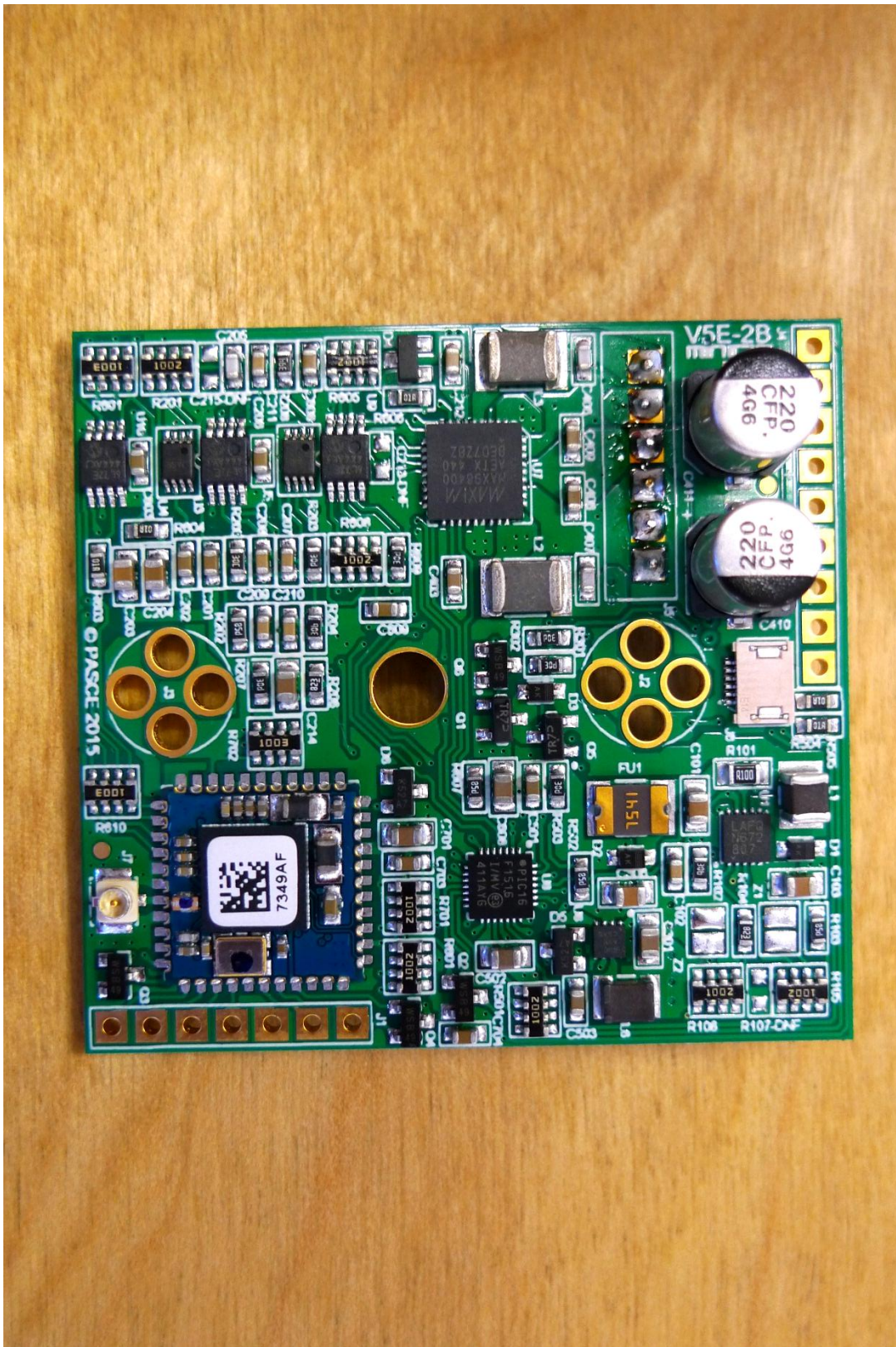
Main PCB Top
