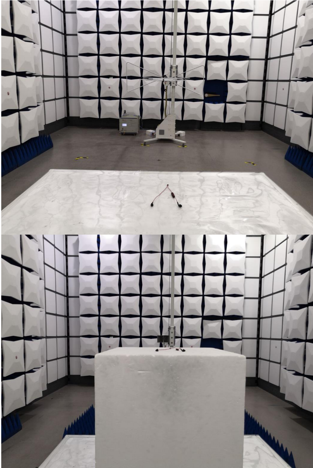
Radiated Emission
