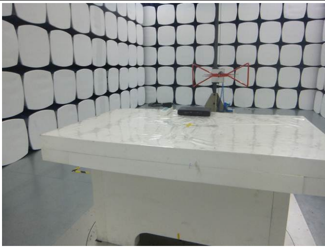
FG9008N Radiated Spurious Emissions Test Setup Below 1GHz
