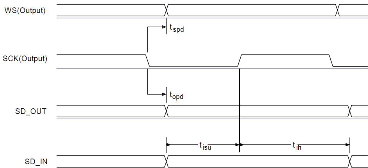
Figure 8.3.3: Digital Audio Interface Master Timing
