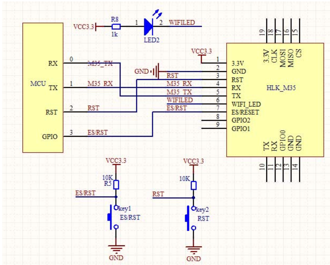
Figure 7. HLK-M35 typical circuit
