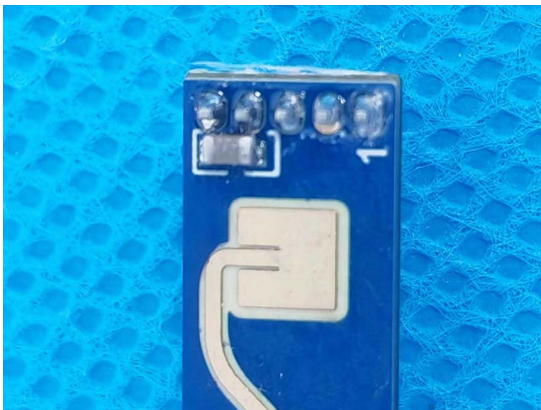
24GHz Radar Antenna_TX
