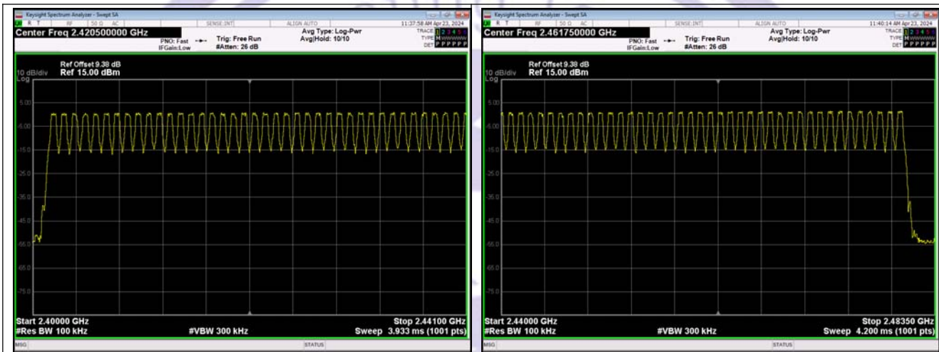
Low End Spectrum Channel Hopping Plot GFSK
