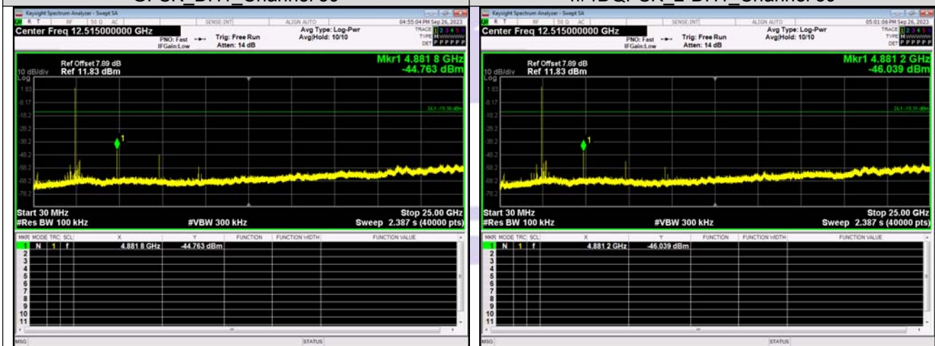
Spurious Emissions
