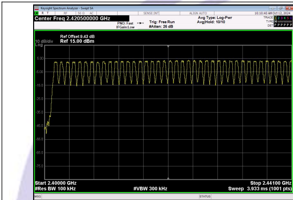
Low End Spectrum Channel Hopping Plot GFSK
