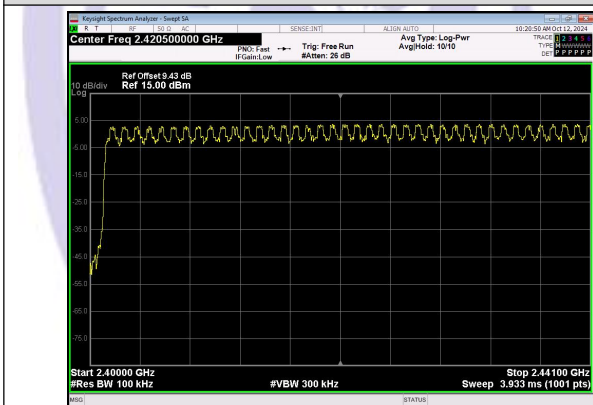
Low End Spectrum Channel Hopping Plot \pi/4 DQPSK
