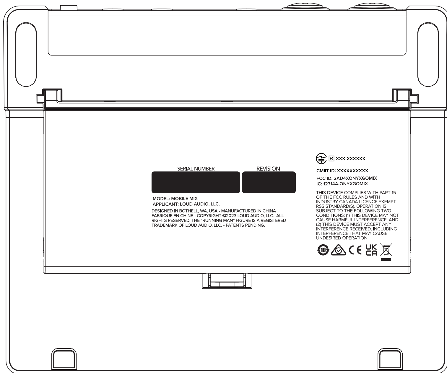
GRAPHIC PLACEMENT ON BOTTOM BATTERY COVER 1:1 SCALE
