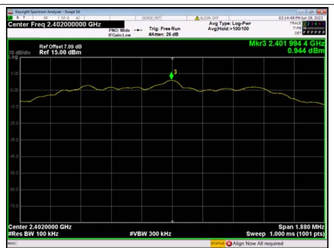
In-Band Reference Level 2LE_Channel 0
