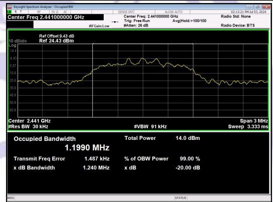
8DPSK_3-DH1_Channel 39
