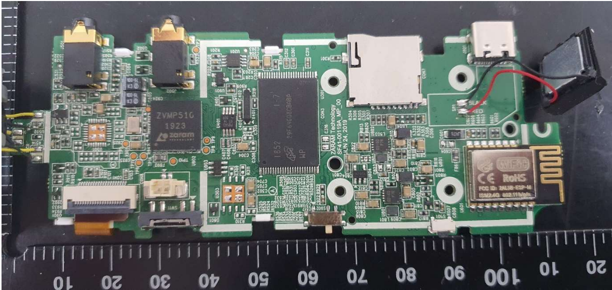
Main Board(Front)
