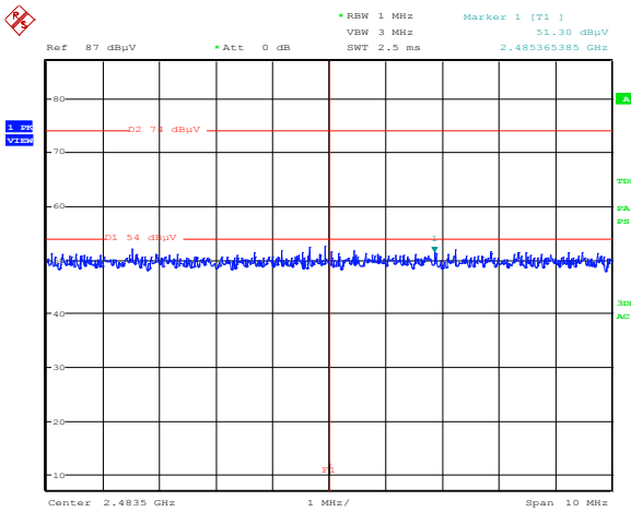
Figure 8.4-5: Upper band edge emission at 2483.5 MHz ( F_1 = 2483.5 MHz)
