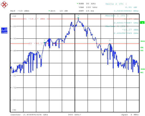
Figure 8.2-1: 20 dB bandwidth (Channel 57)
