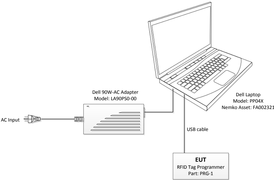
Figure 3.6-1: Setup diagram
