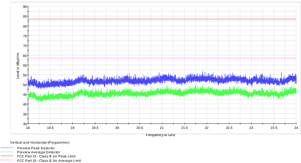
Figure 8.4-3: Spurious emissions above 18 GHz
