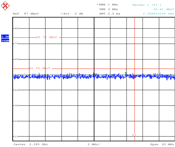
Figure 8.4-4: Lower band edge emission at 2400 MHz ( F_1 = 2400 MHz)
