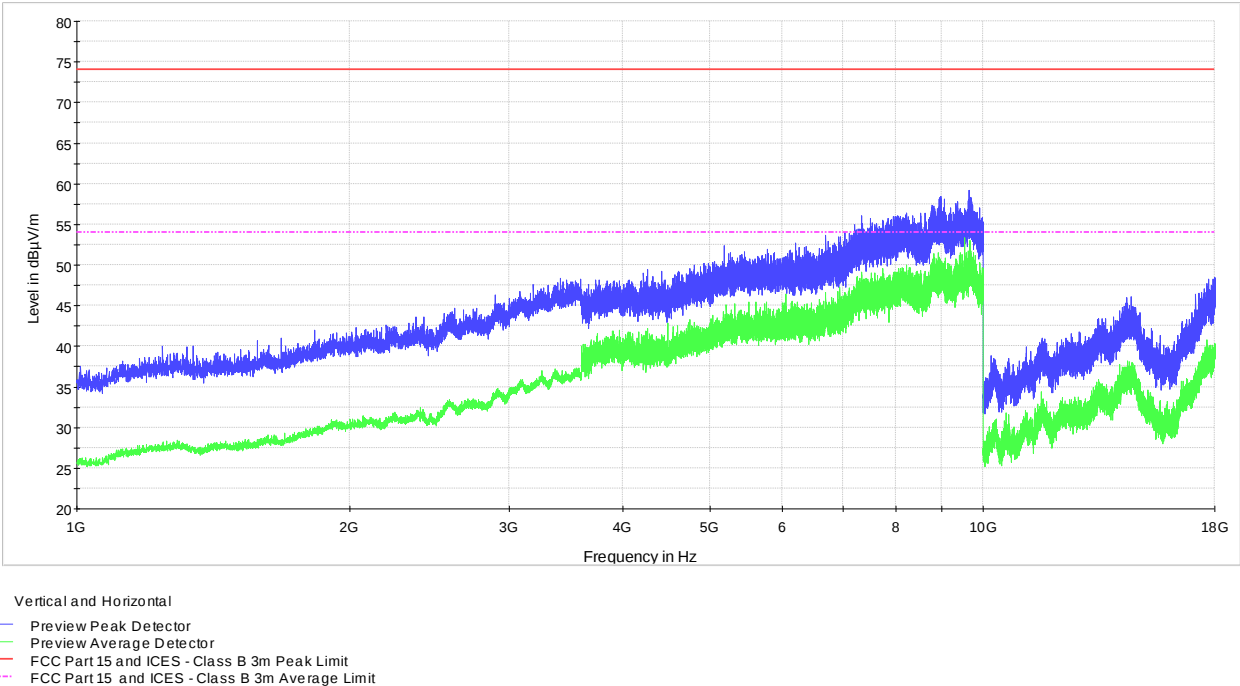
Figure 8.4-2: Spurious emissions within 1–18 GHz
