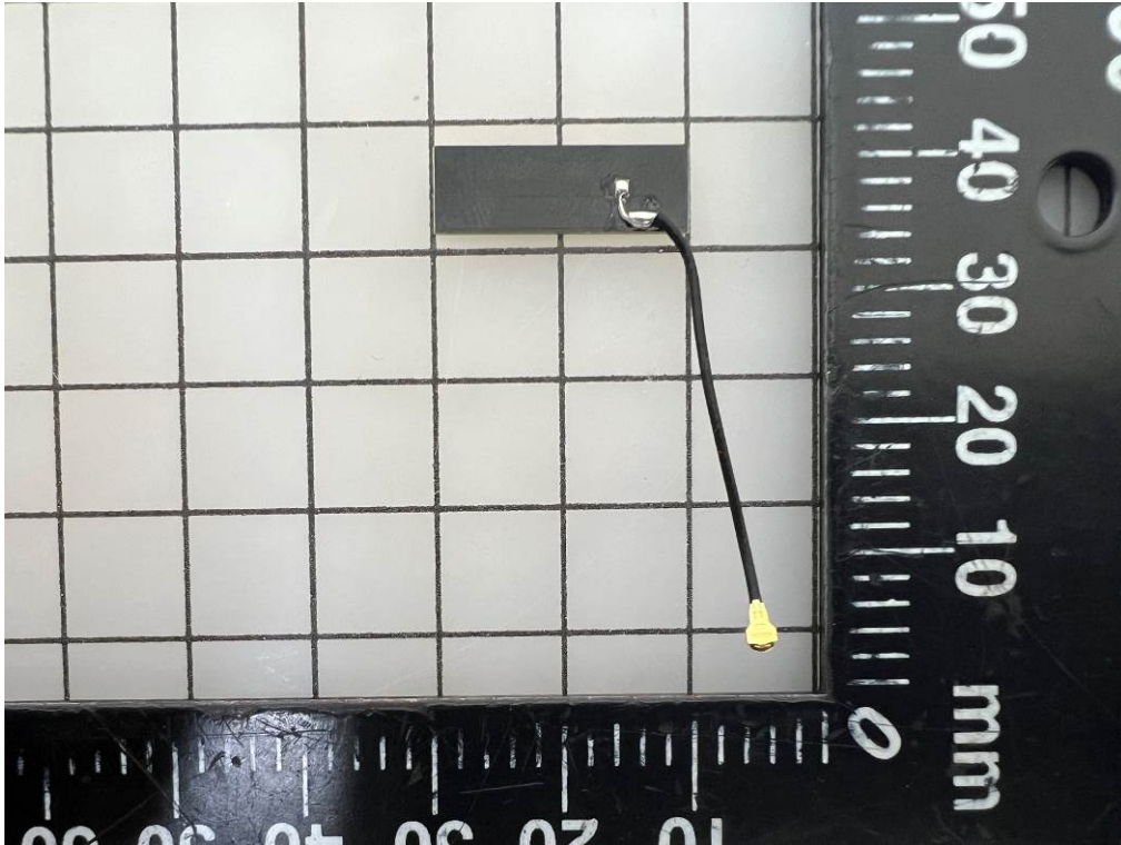
Figure 1 2.4G Antenna
