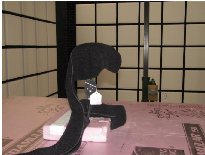
Figure 4: Radiated Emissions – Above 1GHz – Rear View
