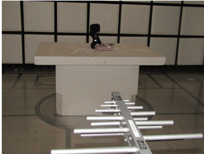
Figure 1: Radiated Emissions – Below 1GHz – Front View
