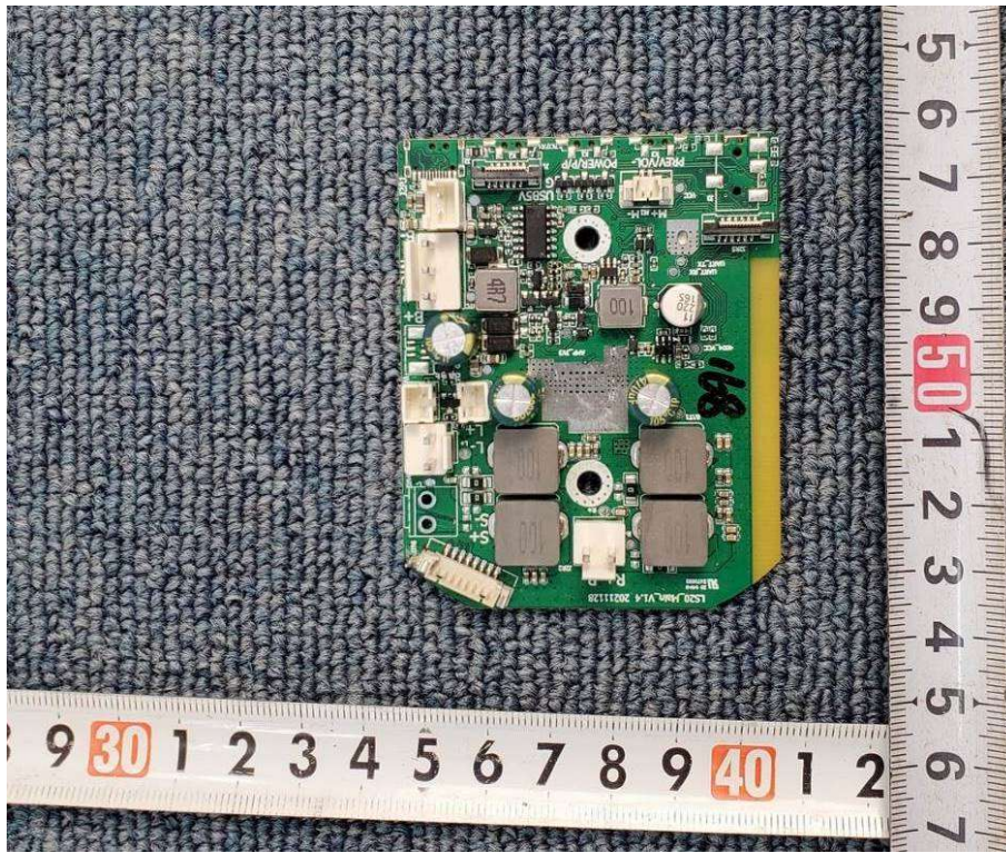
Main Board
