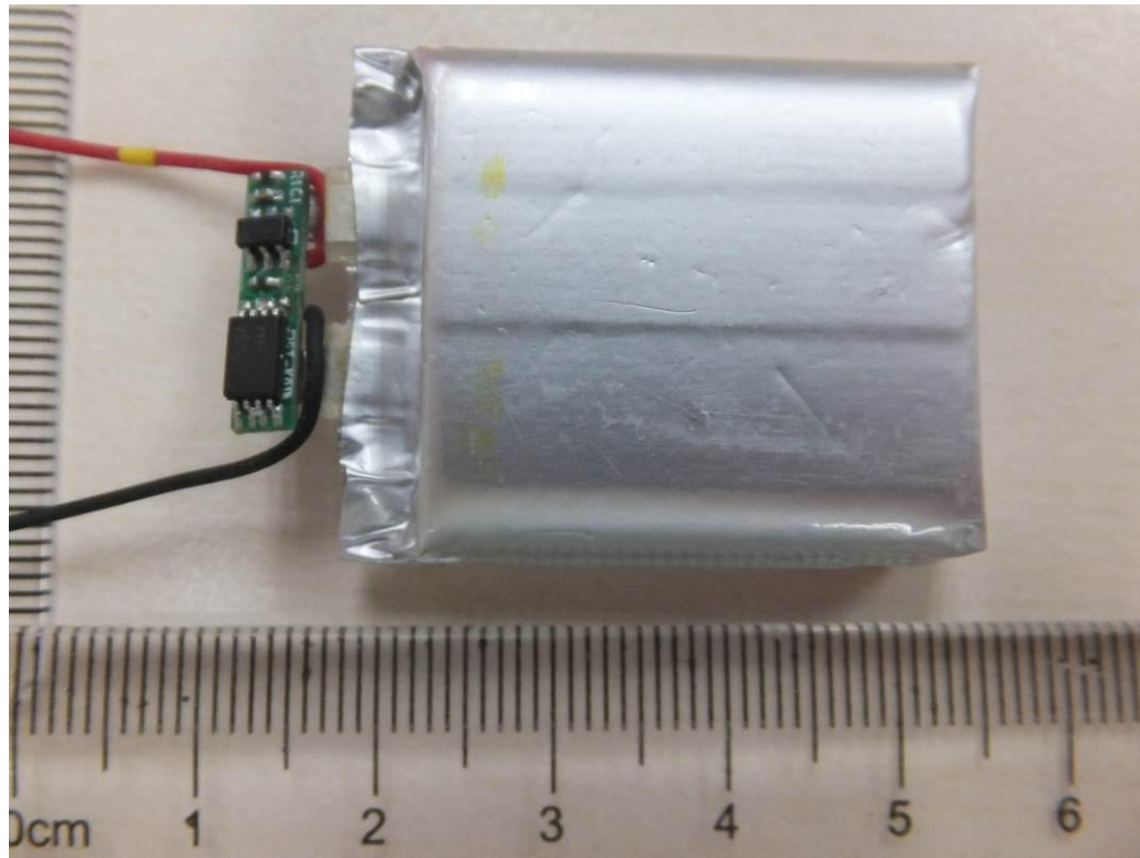
Fig. 7: Internal view
