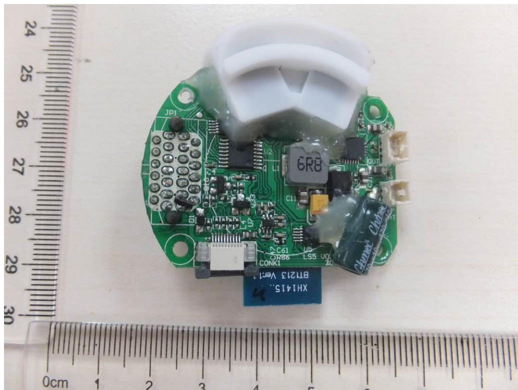
Fig. 4: Internal view
