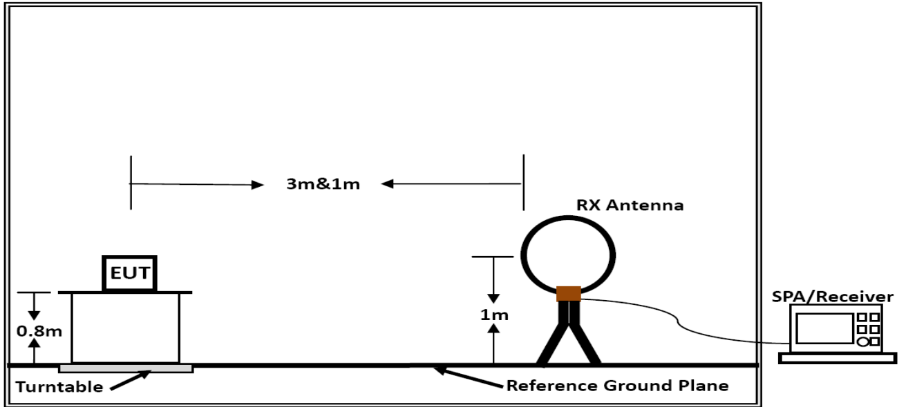
Below 30MHz
