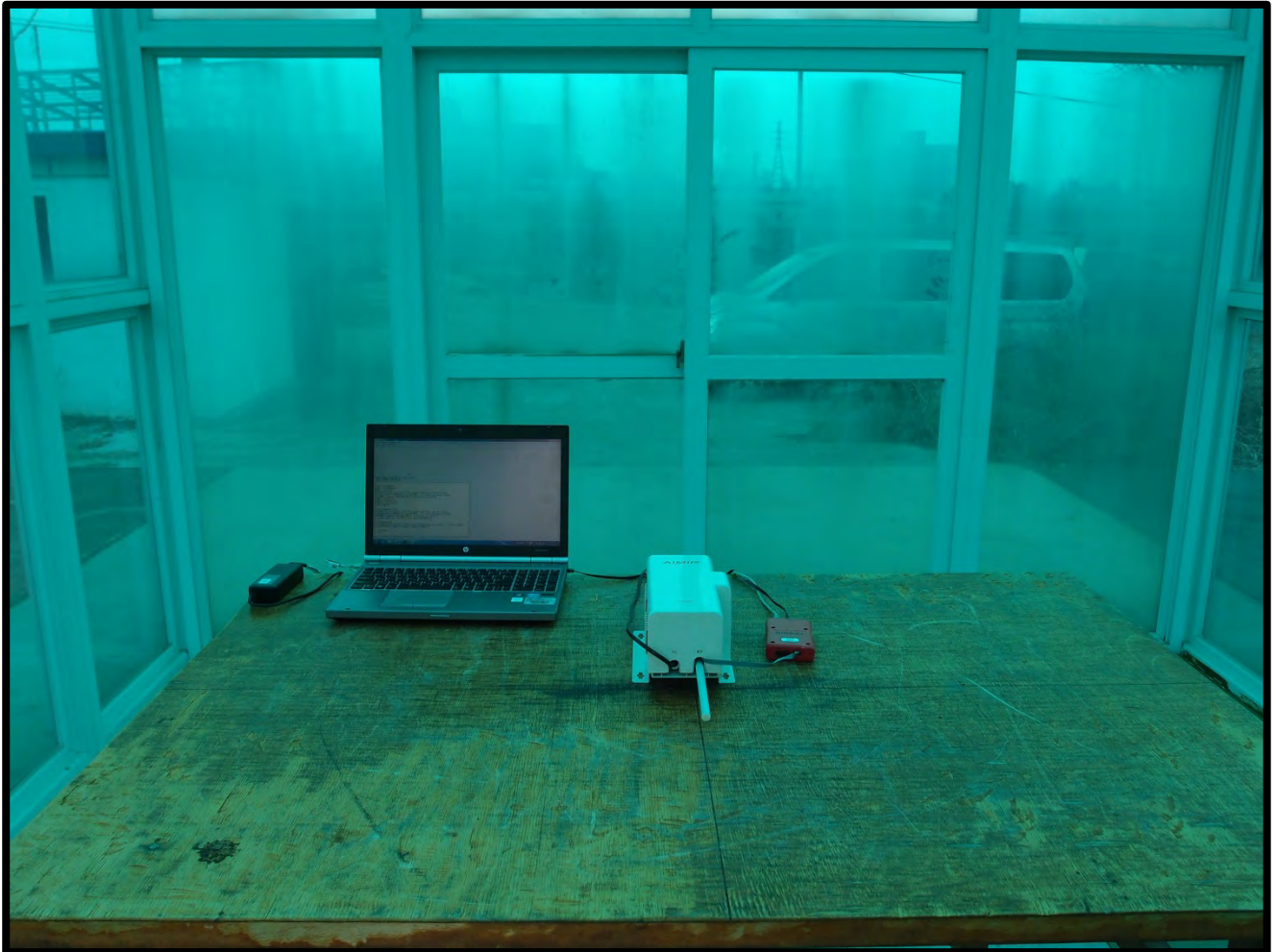
Test Setup of Radiation
