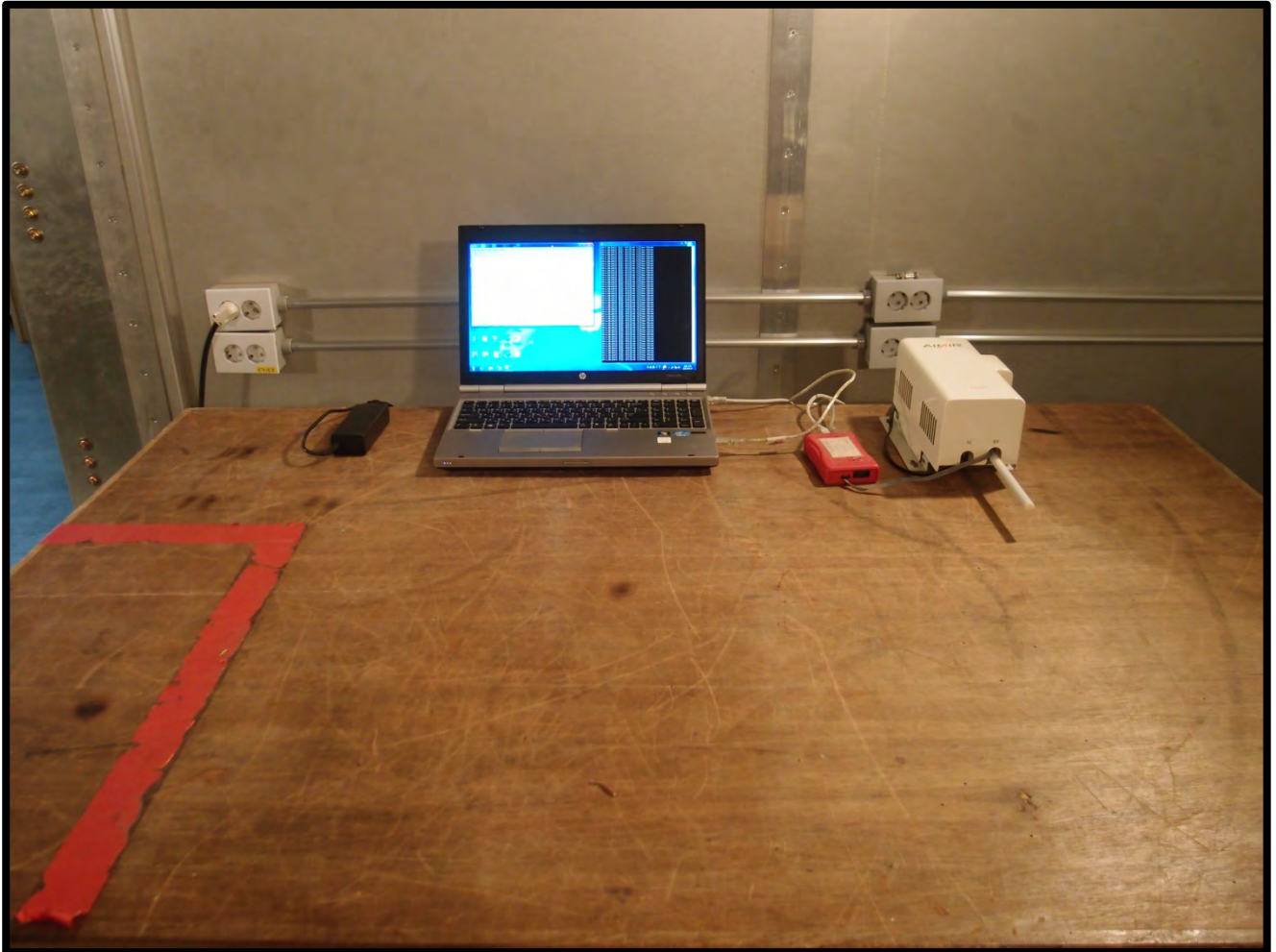
Test Setup of Conducted emission
