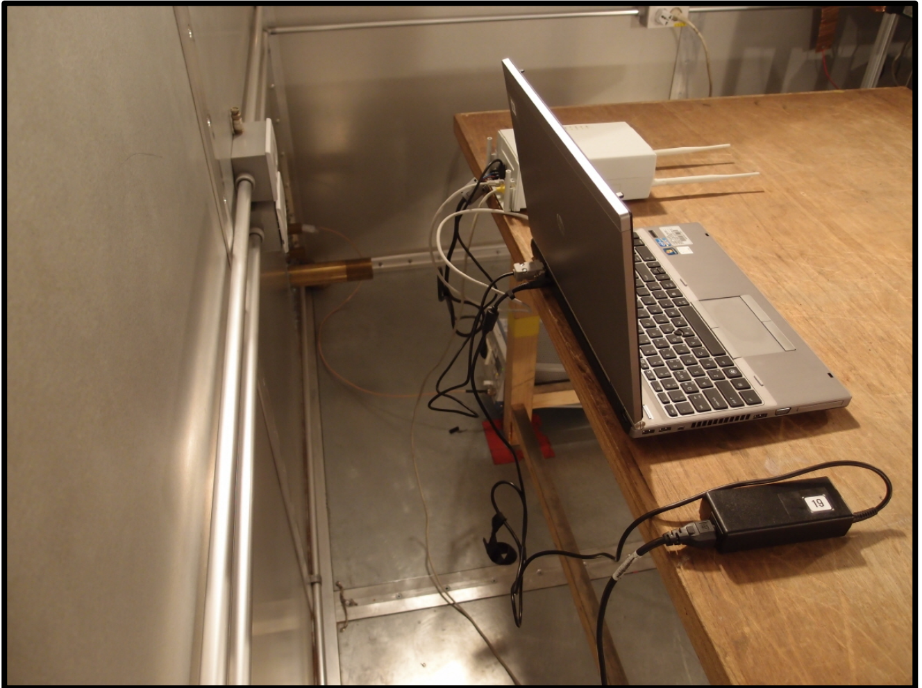
Test Setup of Conducted emission - 2
