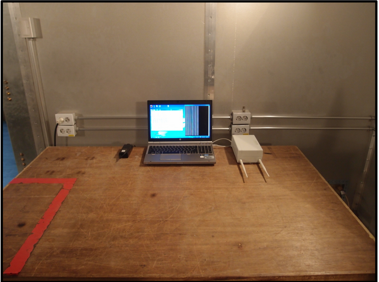
Test Setup of Conducted emission - 1
